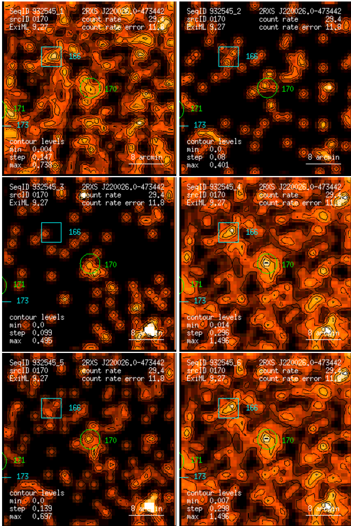
Figure 170: RASS 932545: detection 0170: band rate images, Gaussian filter: (1) PSPC channels 11 – 41, (2) 52 – 90, (3) 91 – 201, (4) 11 – 235, (5) 52 – 201, (6) 11 – 201. Broad band rates in counts/ks. Band rate contour levels in counts/ks/arcmin 2 .
