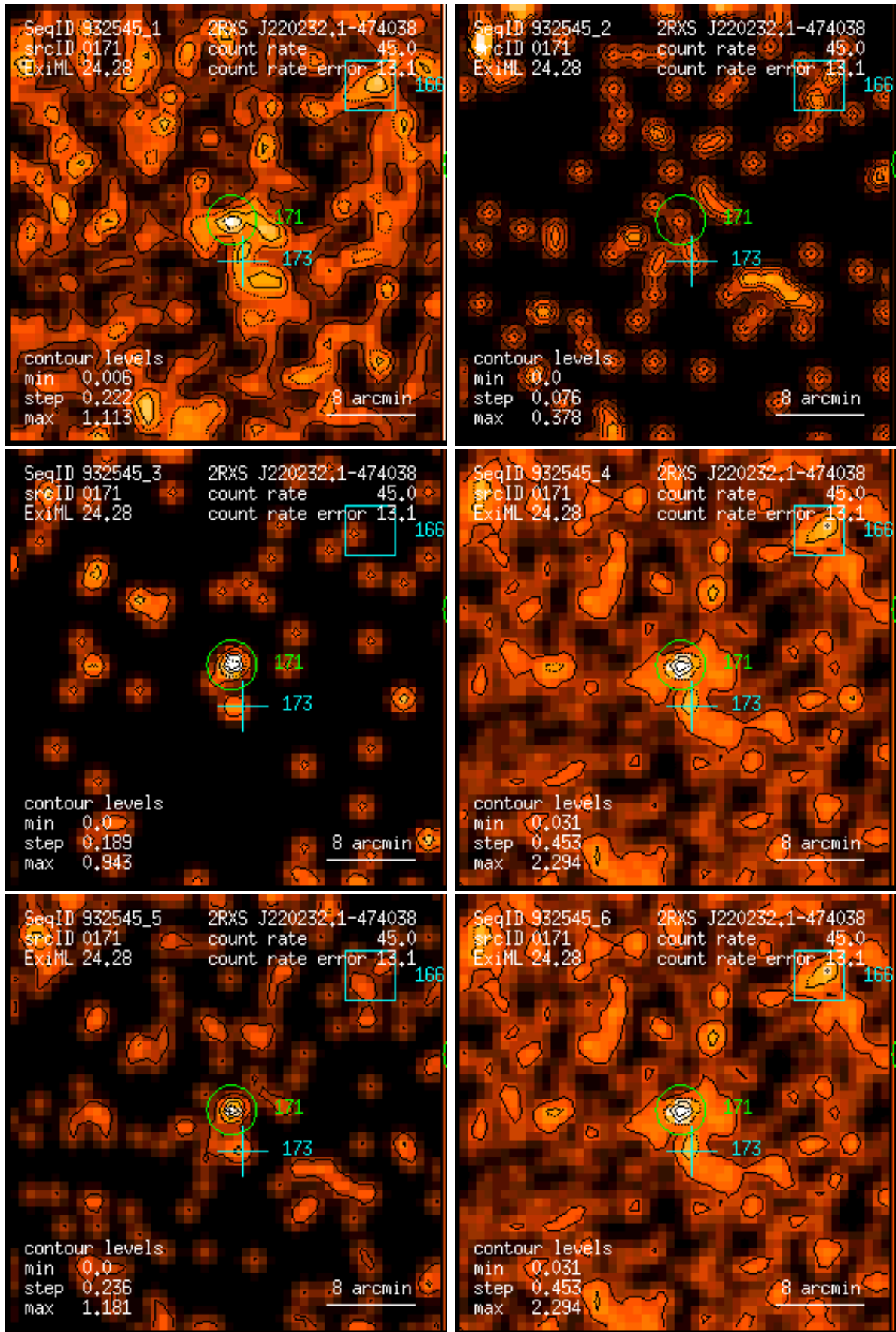
Figure 171: RASS 932545: detection 0171: band rate images, Gaussian filter: (1) PSPC channels 11 – 41, (2) 52 – 90, (3) 91 – 201, (4) 11 – 235, (5) 52 – 201, (6) 11 – 201. Broad band rates in counts/ks. Band rate contour levels in counts/ks/arcmin 2 .
