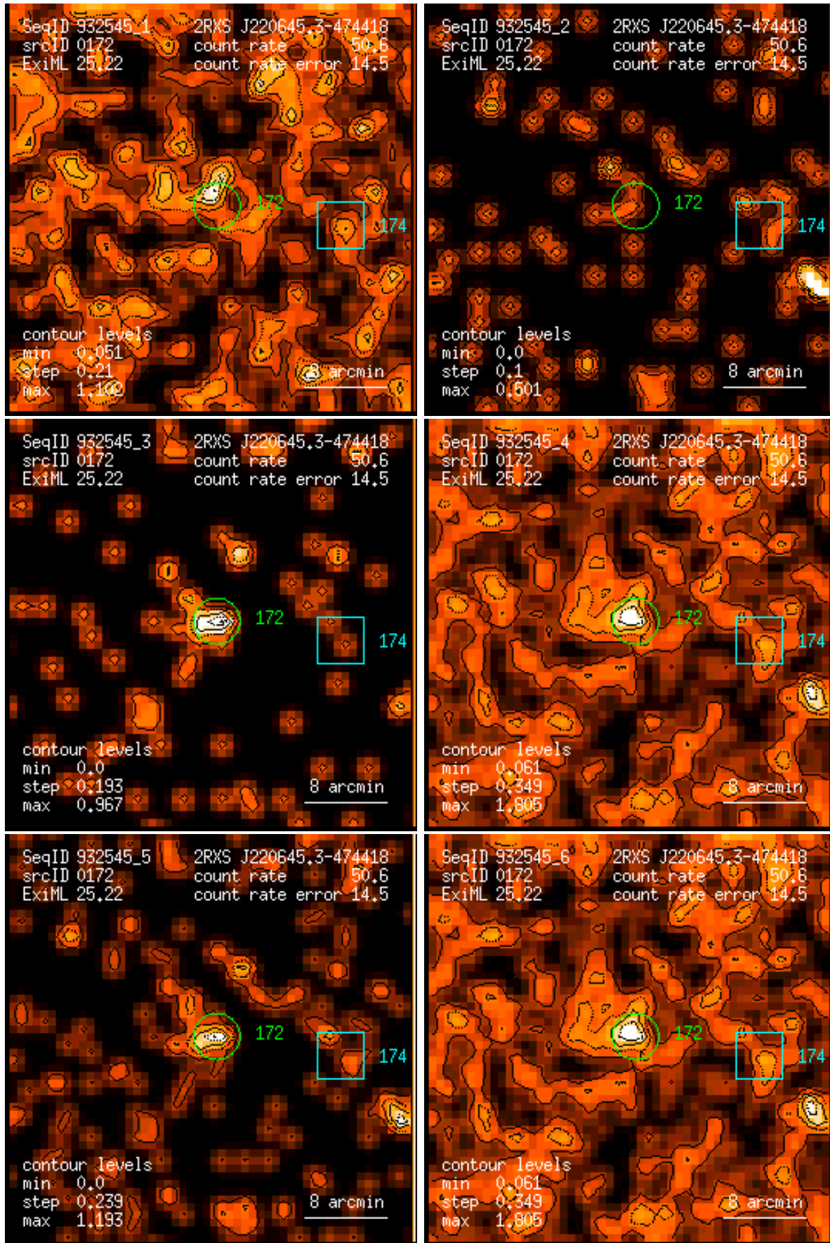
Figure 172: RASS 932545: detection 0172: band rate images, Gaussian filter: (1) PSPC channels 11 – 41, (2) 52 – 90, (3) 91 – 201, (4) 11 – 235, (5) 52 – 201, (6) 11 – 201. Broad band rates in counts/ks. Band rate contour levels in counts/ks/arcmin 2 .
