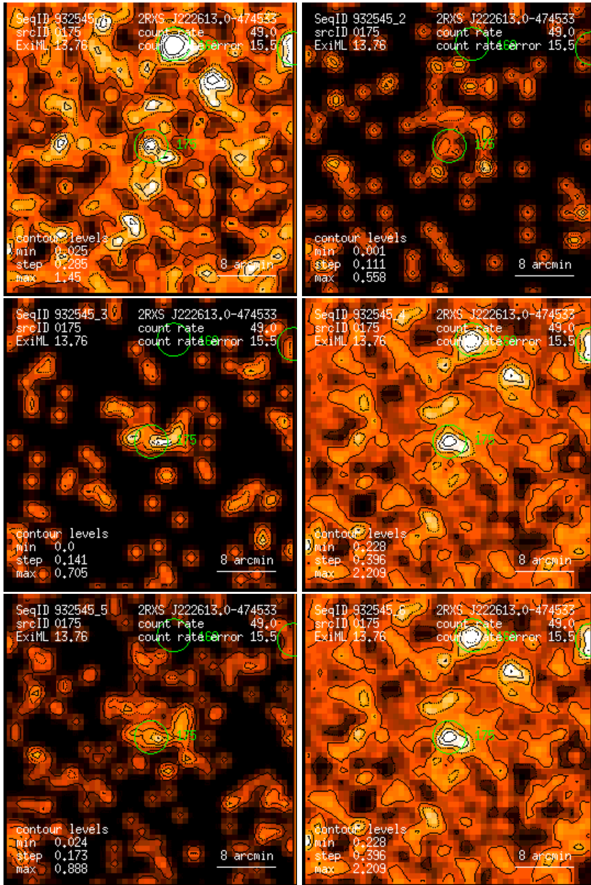
Figure 175: RASS 932545: detection 0175: band rate images, Gaussian filter: (1) PSPC channels 11 – 41, (2) 52 – 90, (3) 91 – 201, (4) 11 – 235, (5) 52 – 201, (6) 11 – 201. Broad band rates in counts/ks. Band rate contour levels in counts/ks/arcmin 2 .
