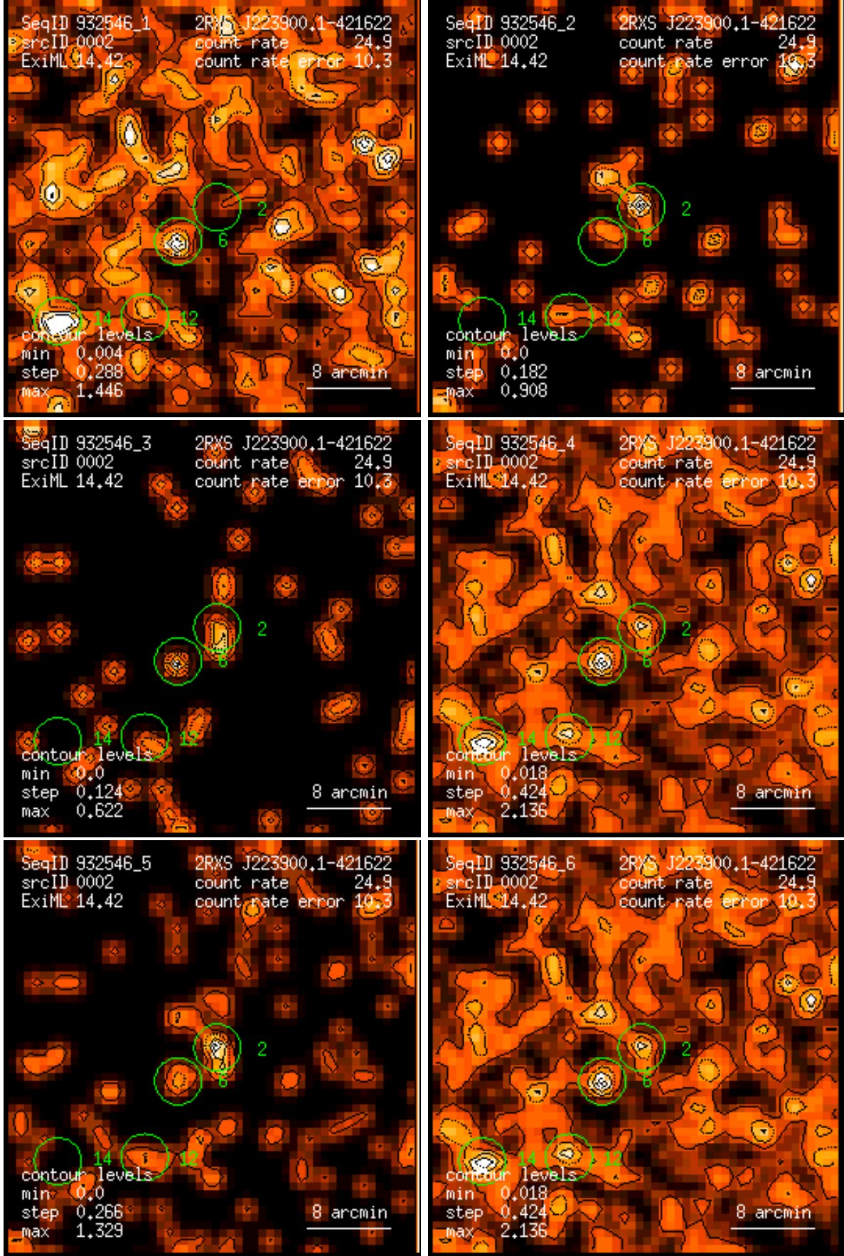
Figure 2: RASS 932546: detection 0002: band rate images, Gaussian filter: (1) PSPC channels 11 – 41, (2) 52 – 90, (3) 91 – 201, (4) 11 – 235, (5) 52 – 201, (6) 11 – 201. Broad band rates in counts/ks. Band rate contour levels in counts/ks/arcmin 2 .
