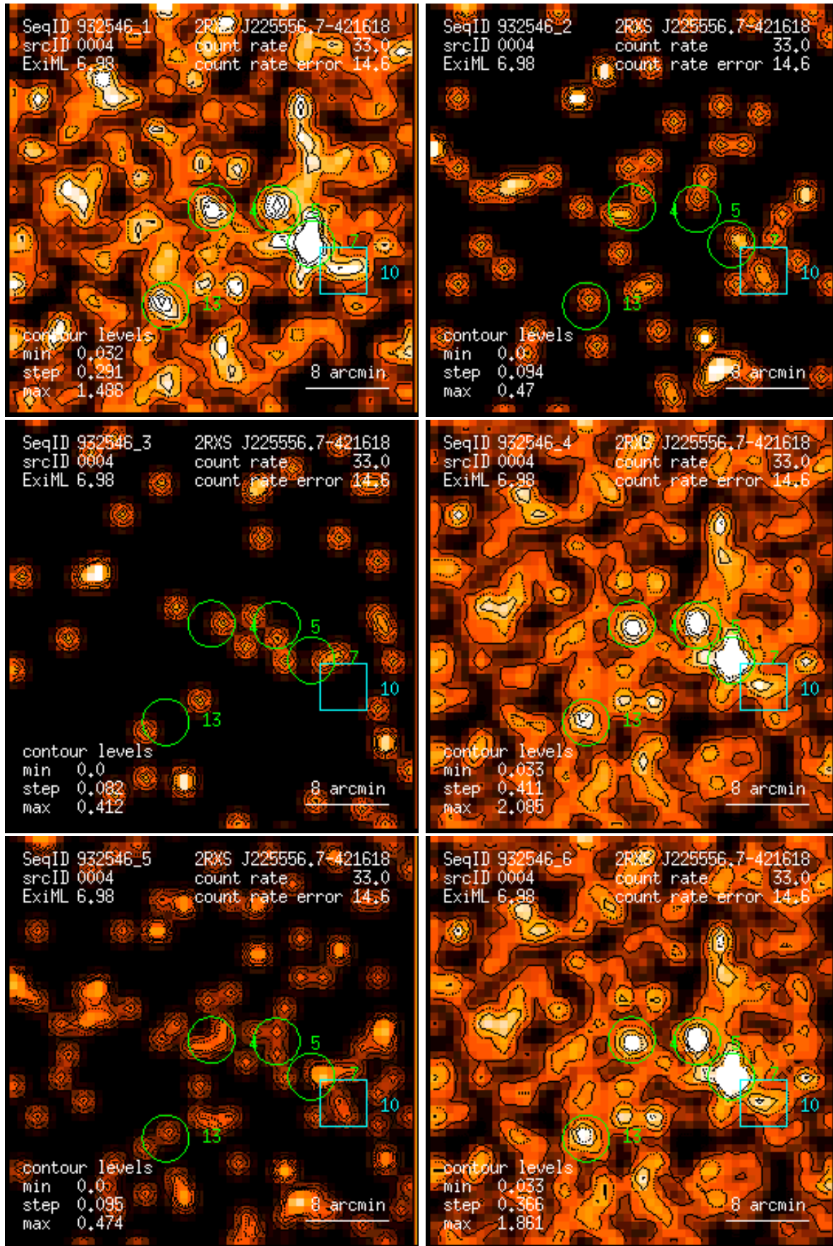
Figure 4: RASS 932546: detection 0004: band rate images, Gaussian filter: (1) PSPC channels 11 – 41, (2) 52 – 90, (3) 91 – 201, (4) 11 – 235, (5) 52 – 201, (6) 11 – 201. Broad band rates in counts/ks. Band rate contour levels in counts/ks/arcmin 2 .
