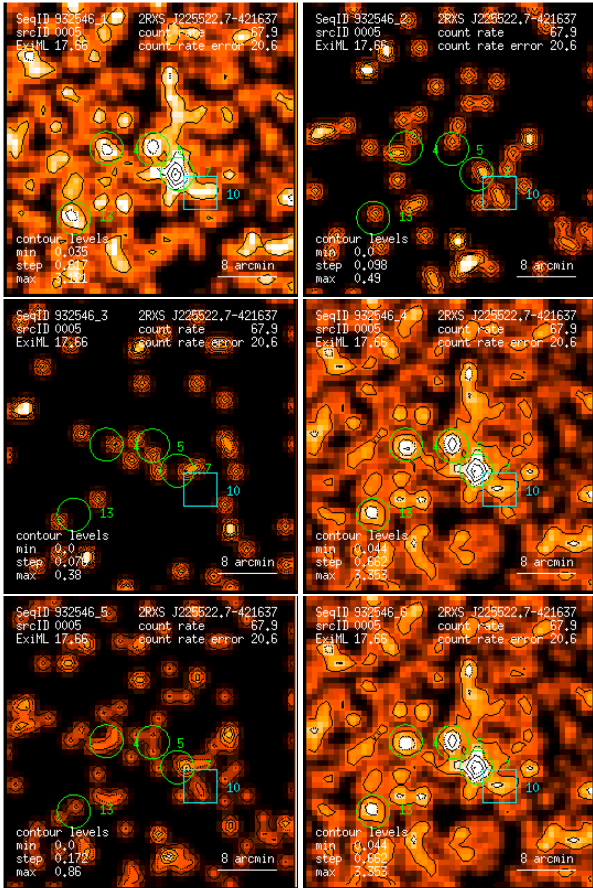
Figure 5: RASS 932546: detection 0005: band rate images, Gaussian filter: (1) PSPC channels 11 – 41, (2) 52 – 90, (3) 91 – 201, (4) 11 – 235, (5) 52 – 201, (6) 11 – 201. Broad band rates in counts/ks. Band rate contour levels in counts/ks/arcmin 2 .
