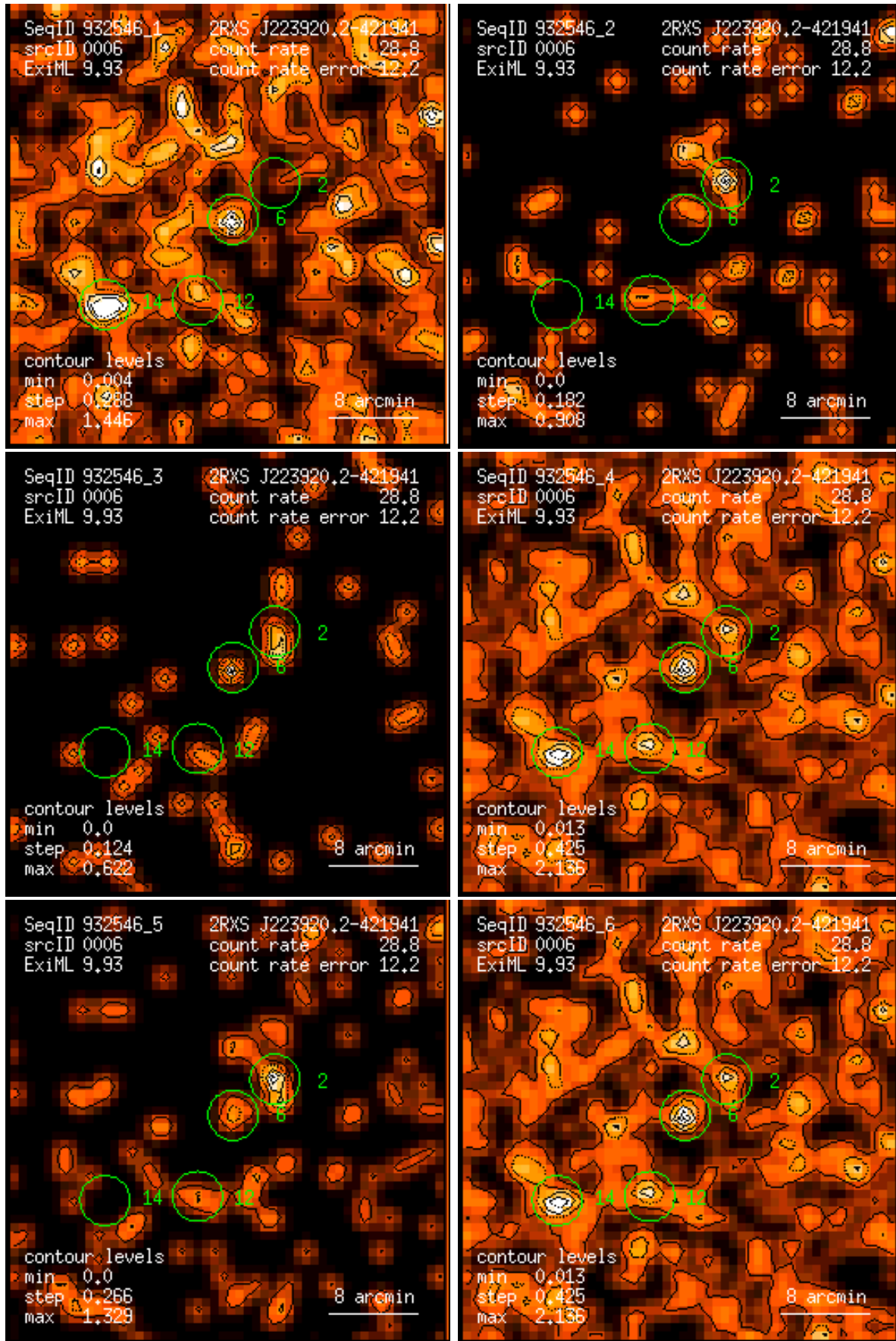
Figure 6: RASS 932546: detection 0006: band rate images, Gaussian filter: (1) PSPC channels 11 – 41, (2) 52 – 90, (3) 91 – 201, (4) 11 – 235, (5) 52 – 201, (6) 11 – 201. Broad band rates in counts/ks. Band rate contour levels in counts/ks/arcmin 2 .
