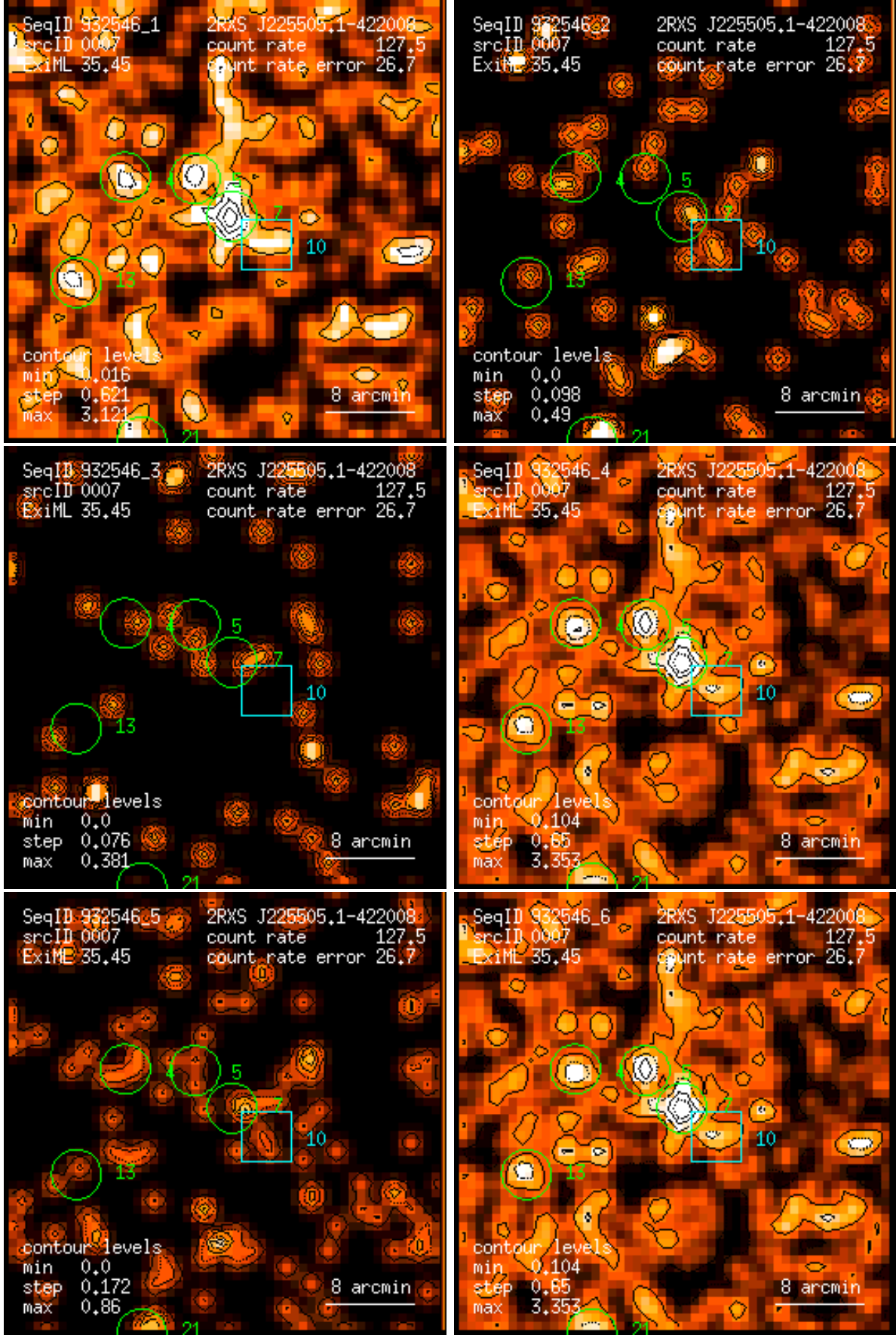
Figure 7: RASS 932546: detection 0007: band rate images, Gaussian filter: (1) PSPC channels 11 – 41, (2) 52 – 90, (3) 91 – 201, (4) 11 – 235, (5) 52 – 201, (6) 11 – 201. Broad band rates in counts/ks. Band rate contour levels in counts/ks/arcmin 2 .
