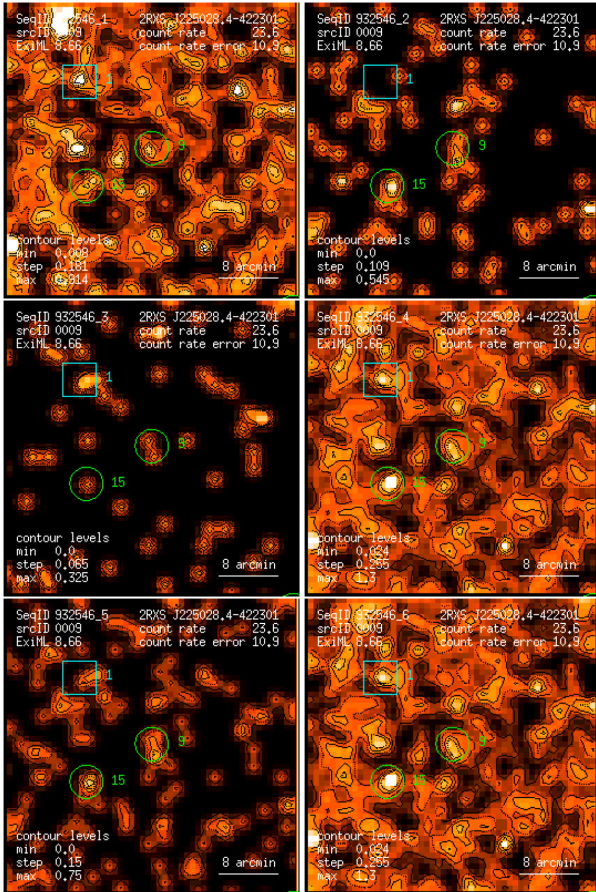
Figure 9: RASS 932546: detection 0009: band rate images, Gaussian filter: (1) PSPC channels 11 – 41, (2) 52 – 90, (3) 91 – 201, (4) 11 – 235, (5) 52 – 201, (6) 11 – 201. Broad band rates in counts/ks. Band rate contour levels in counts/ks/arcmin 2 .
