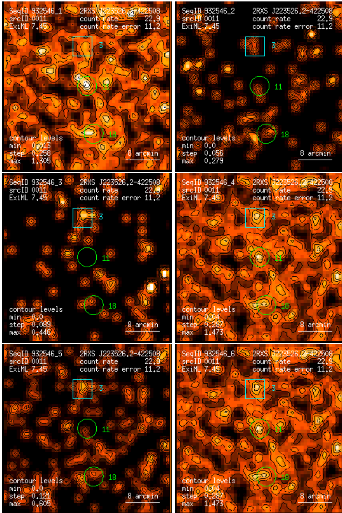
Figure 11: RASS 932546: detection 0011: band rate images, Gaussian filter: (1) PSPC channels 11 – 41, (2) 52 – 90, (3) 91 – 201, (4) 11 – 235, (5) 52 – 201, (6) 11 – 201. Broad band rates in counts/ks. Band rate contour levels in counts/ks/arcmin 2 .
