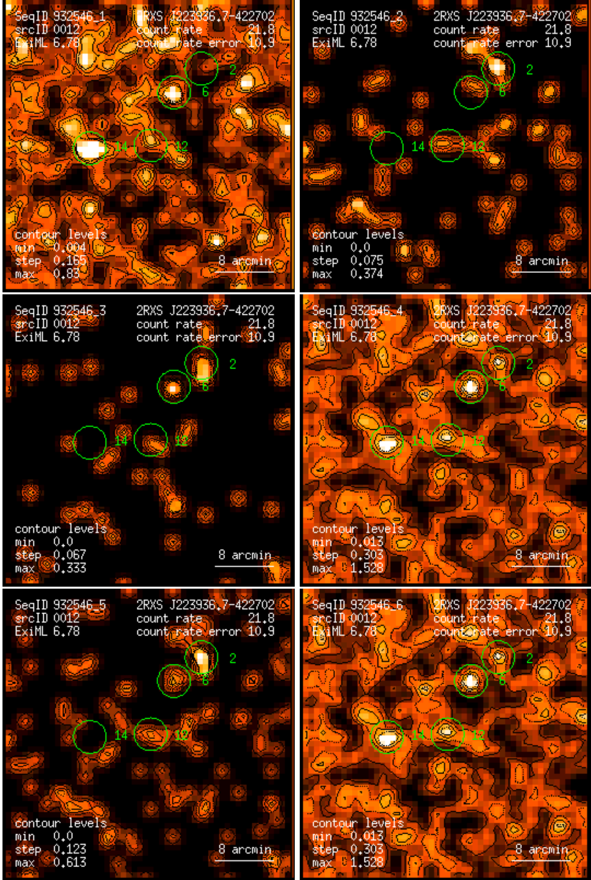
Figure 12: RASS 932546: detection 0012: band rate images, Gaussian filter: (1) PSPC channels 11 – 41, (2) 52 – 90, (3) 91 – 201, (4) 11 – 235, (5) 52 – 201, (6) 11 – 201. Broad band rates in counts/ks. Band rate contour levels in counts/ks/arcmin 2 .
