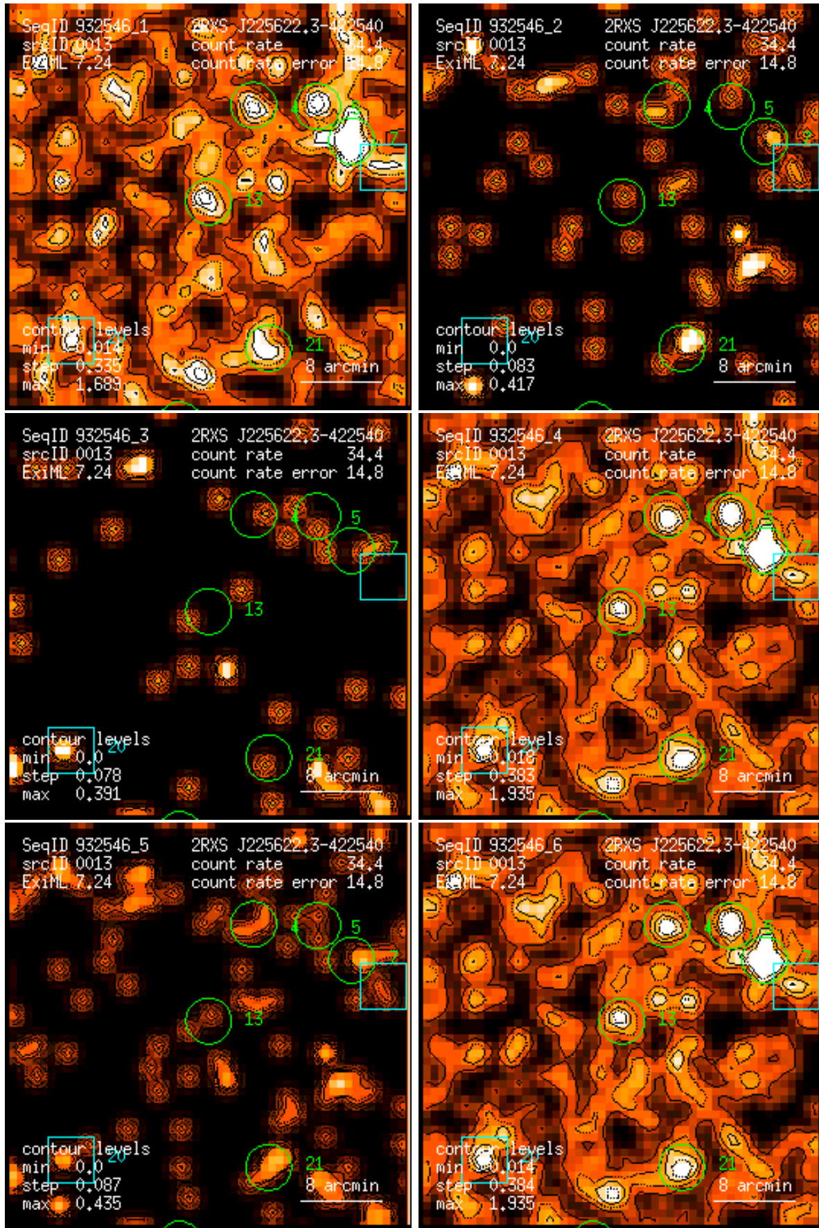
Figure 13: RASS 932546: detection 0013: band rate images, Gaussian filter: (1) PSPC channels 11 – 41, (2) 52 – 90, (3) 91 – 201, (4) 11 – 235, (5) 52 – 201, (6) 11 – 201. Broad band rates in counts/ks. Band rate contour levels in counts/ks/arcmin 2 .
