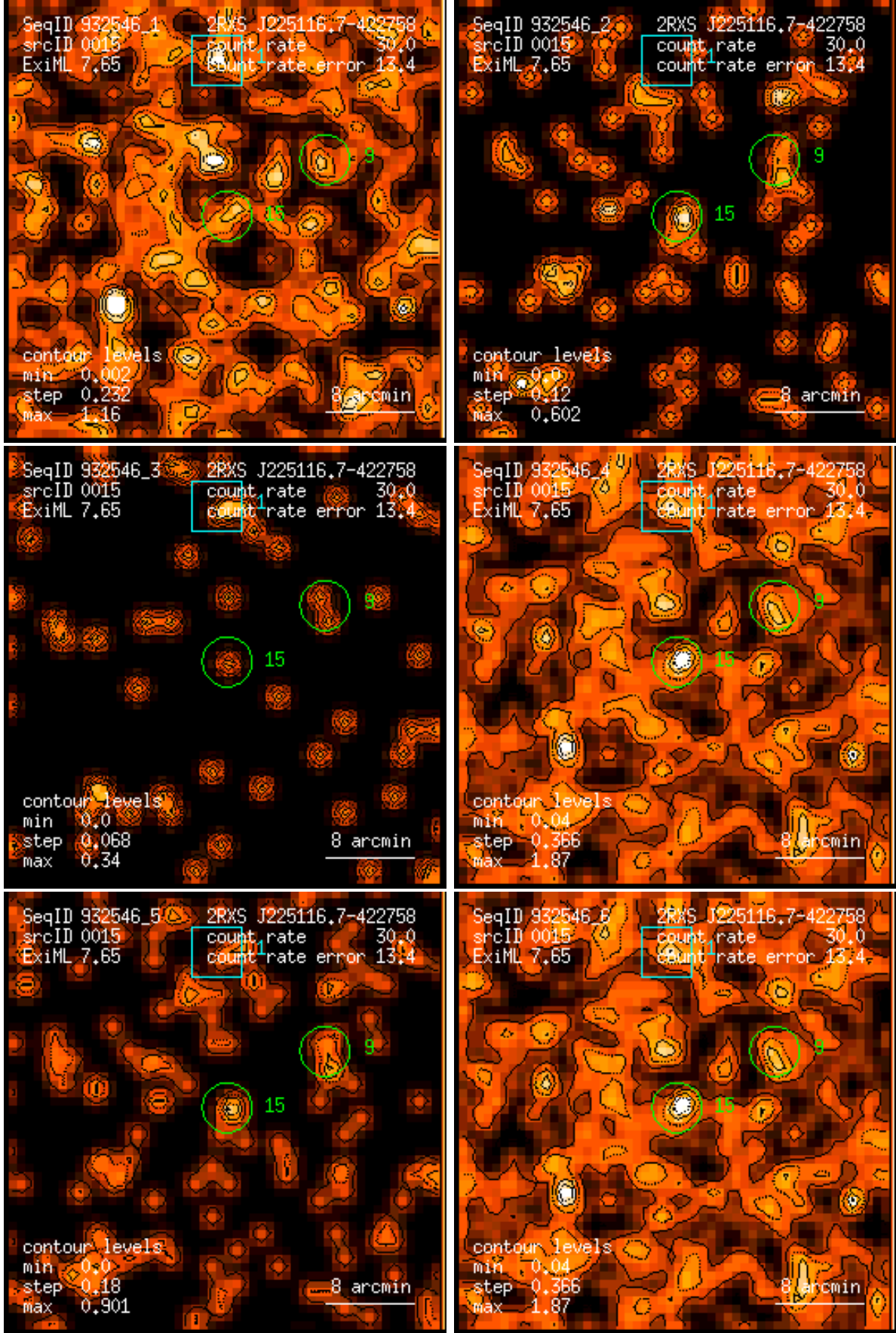
Figure 15: RASS 932546: detection 0015: band rate images, Gaussian filter: (1) PSPC channels 11 – 41, (2) 52 – 90, (3) 91 – 201, (4) 11 – 235, (5) 52 – 201, (6) 11 – 201. Broad band rates in counts/ks. Band rate contour levels in counts/ks/arcmin 2 .
