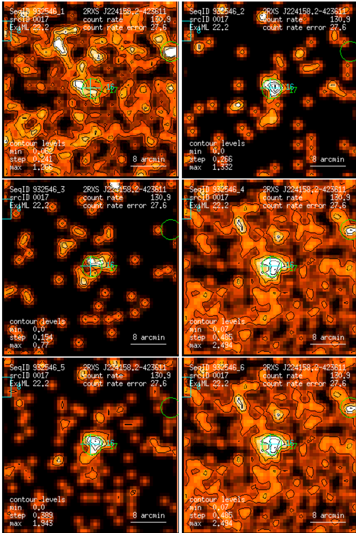
Figure 17: RASS 932546: detection 0017: band rate images, Gaussian filter: (1) PSPC channels 11 – 41, (2) 52 – 90, (3) 91 – 201, (4) 11 – 235, (5) 52 – 201, (6) 11 – 201. Broad band rates in counts/ks. Band rate contour levels in counts/ks/arcmin 2 .
