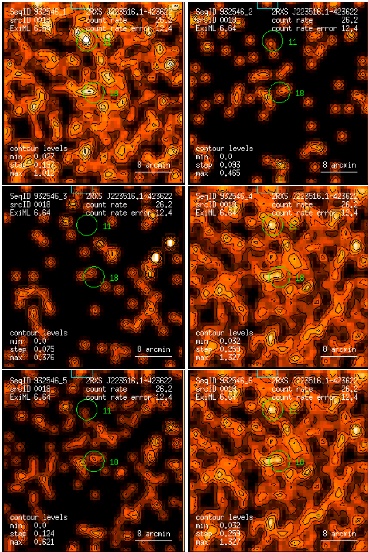
Figure 18: RASS 932546: detection 0018: band rate images, Gaussian filter: (1) PSPC channels 11 – 41, (2) 52 – 90, (3) 91 – 201, (4) 11 – 235, (5) 52 – 201, (6) 11 – 201. Broad band rates in counts/ks. Band rate contour levels in counts/ks/arcmin 2 .
