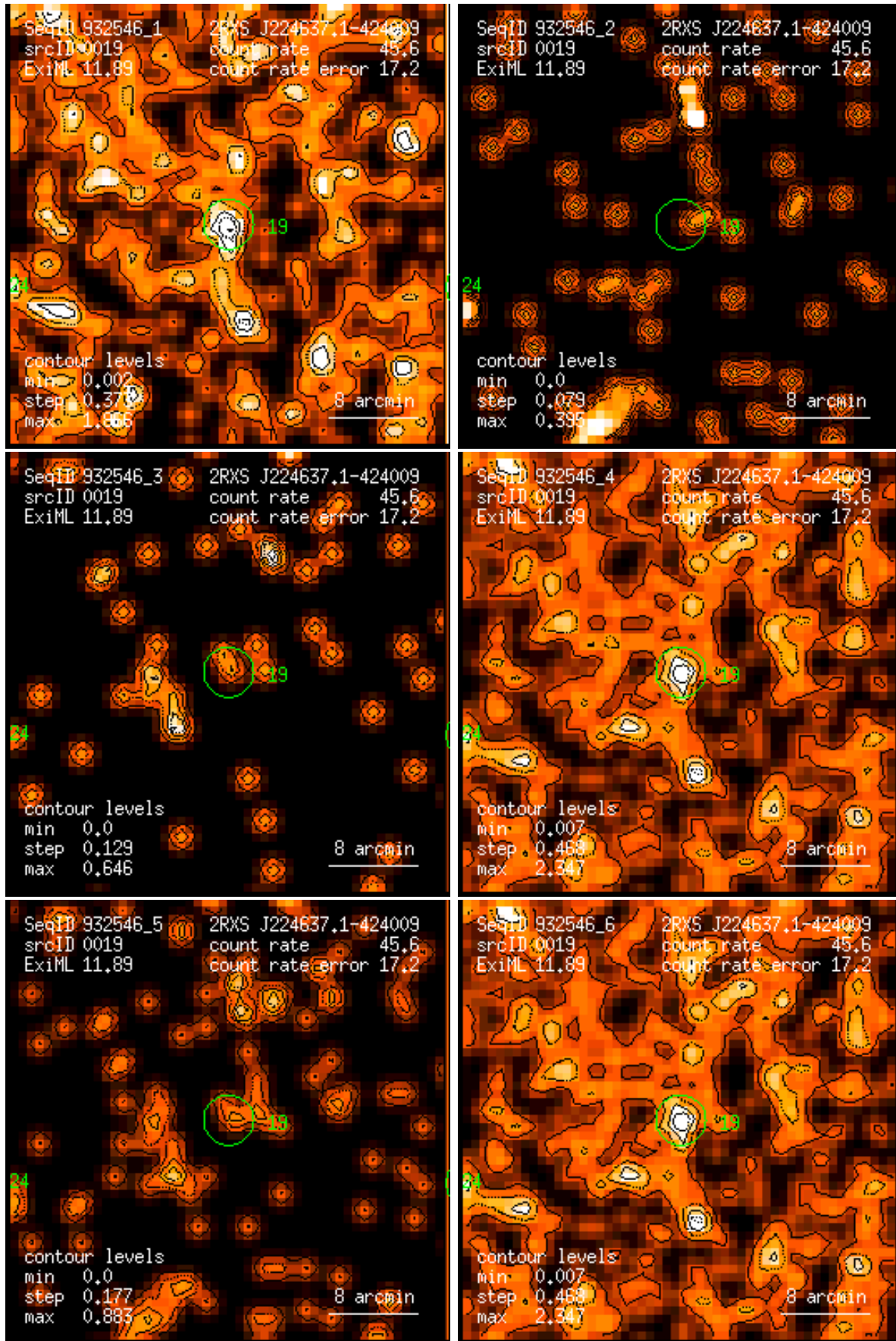
Figure 19: RASS 932546: detection 0019: band rate images, Gaussian filter: (1) PSPC channels 11 – 41, (2) 52 – 90, (3) 91 – 201, (4) 11 – 235, (5) 52 – 201, (6) 11 – 201. Broad band rates in counts/ks. Band rate contour levels in counts/ks/arcmin 2 .
