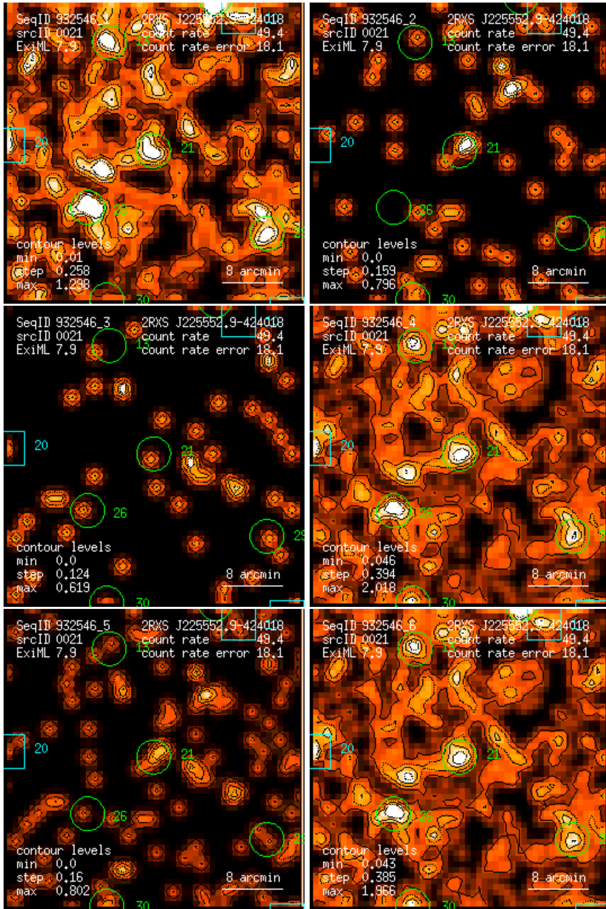
Figure 21: RASS 932546: detection 0021: band rate images, Gaussian filter: (1) PSPC channels 11 – 41, (2) 52 – 90, (3) 91 – 201, (4) 11 – 235, (5) 52 – 201, (6) 11 – 201. Broad band rates in counts/ks. Band rate contour levels in counts/ks/arcmin 2 .
