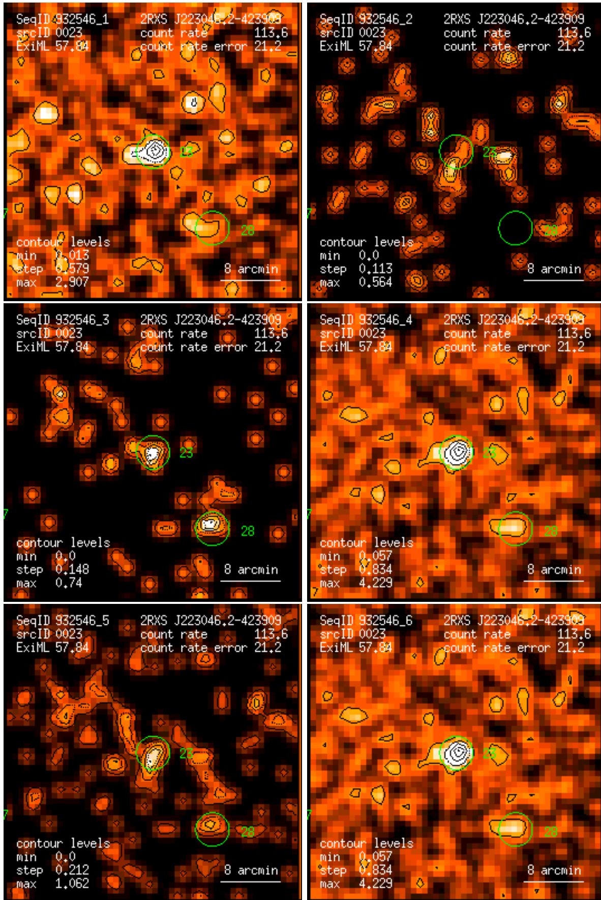
Figure 23: RASS 932546: detection 0023: band rate images, Gaussian filter: (1) PSPC channels 11 – 41, (2) 52 – 90, (3) 91 – 201, (4) 11 – 235, (5) 52 – 201, (6) 11 – 201. Broad band rates in counts/ks. Band rate contour levels in counts/ks/arcmin 2 .
