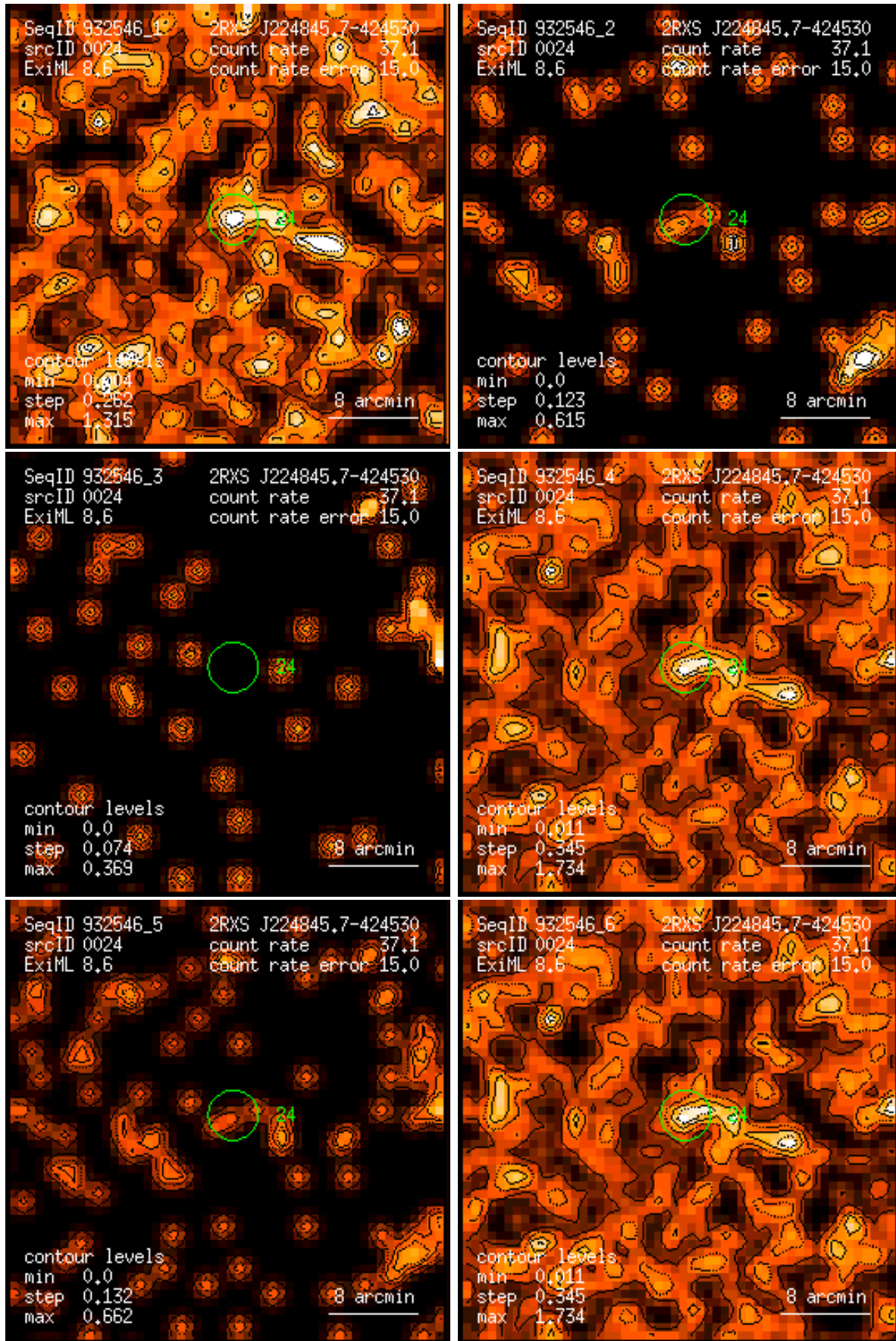
Figure 24: RASS 932546: detection 0024: band rate images, Gaussian filter: (1) PSPC channels 11 – 41, (2) 52 – 90, (3) 91 – 201, (4) 11 – 235, (5) 52 – 201, (6) 11 – 201. Broad band rates in counts/ks. Band rate contour levels in counts/ks/arcmin 2 .
