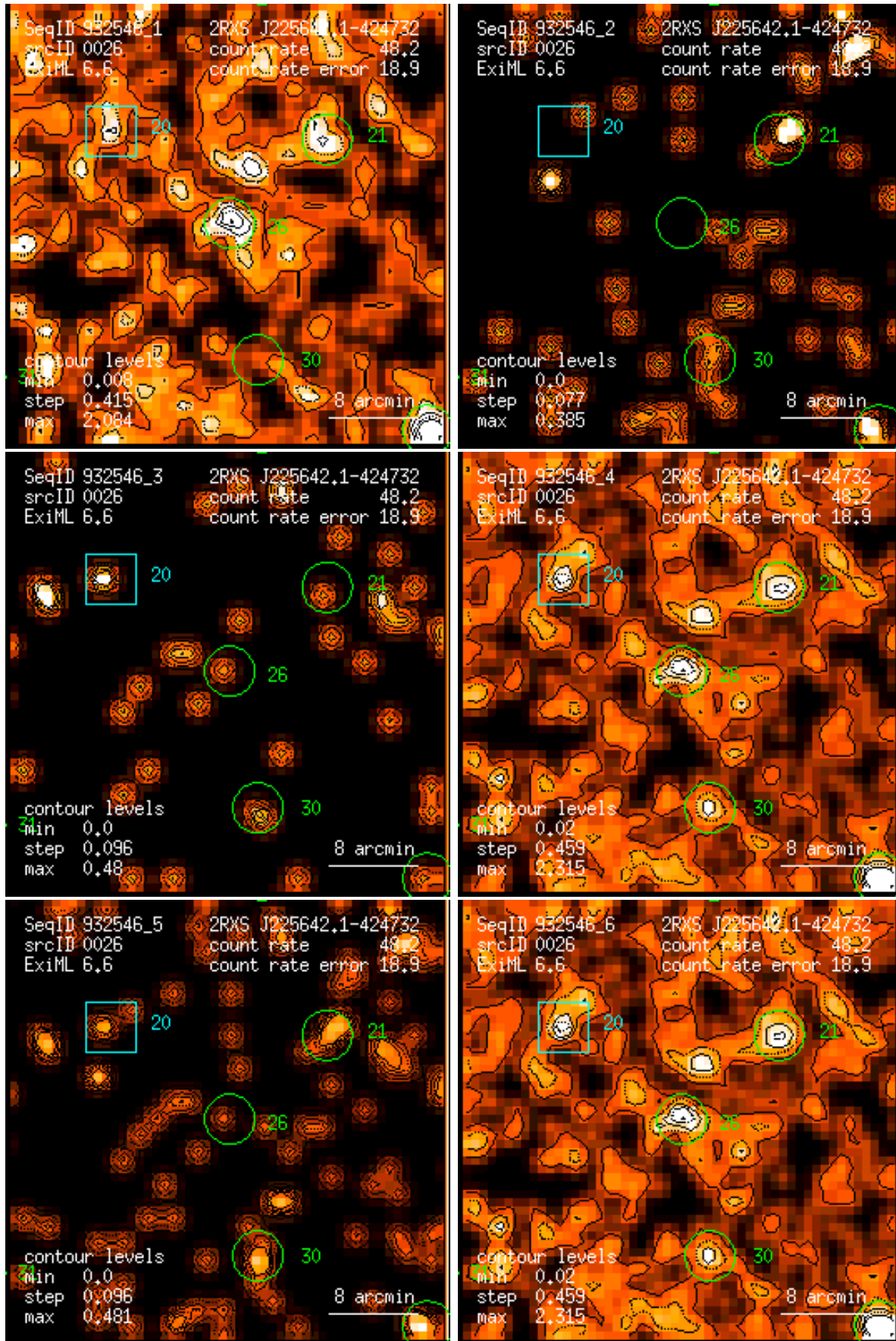
Figure 26: RASS 932546: detection 0026: band rate images, Gaussian filter: (1) PSPC channels 11 – 41, (2) 52 – 90, (3) 91 – 201, (4) 11 – 235, (5) 52 – 201, (6) 11 – 201. Broad band rates in counts/ks. Band rate contour levels in counts/ks/arcmin 2 .
