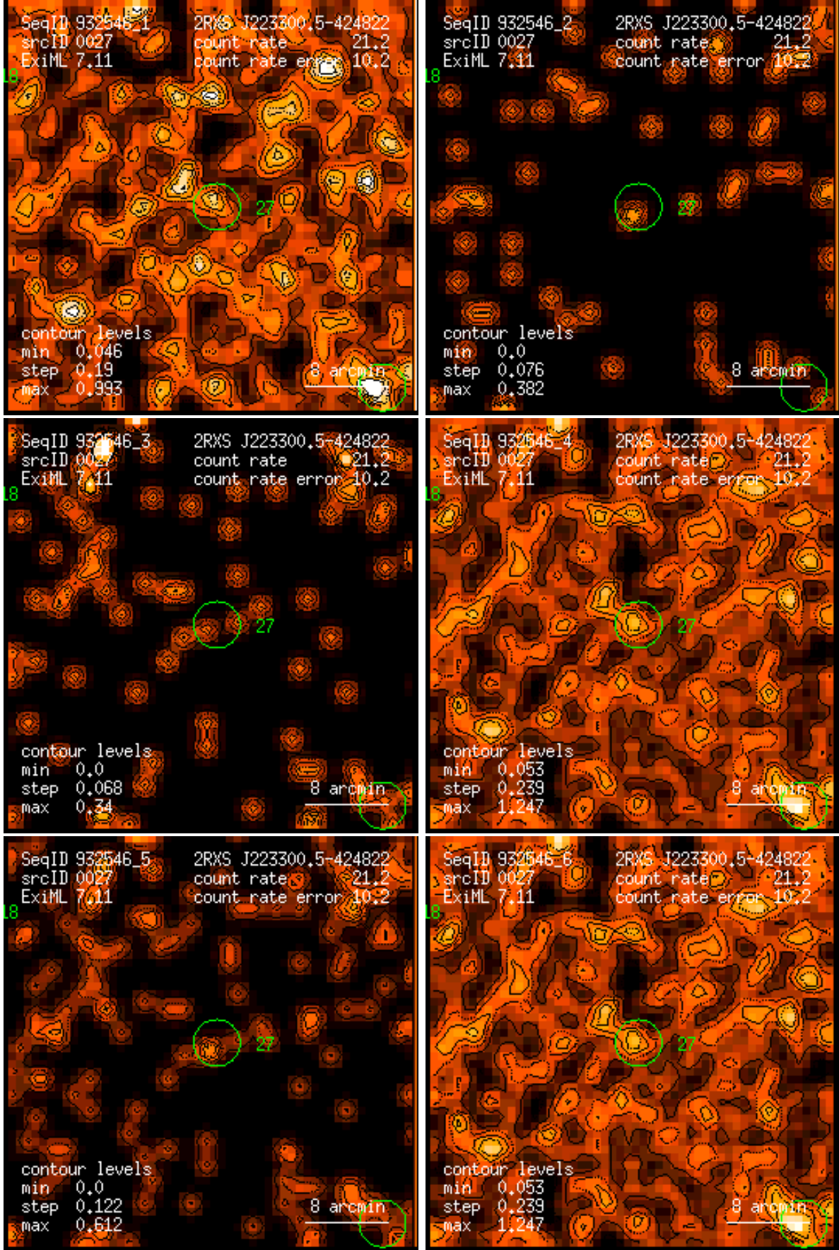
Figure 27: RASS 932546: detection 0027: band rate images, Gaussian filter: (1) PSPC channels 11 – 41, (2) 52 – 90, (3) 91 – 201, (4) 11 – 235, (5) 52 – 201, (6) 11 – 201. Broad band rates in counts/ks. Band rate contour levels in counts/ks/arcmin 2 .
