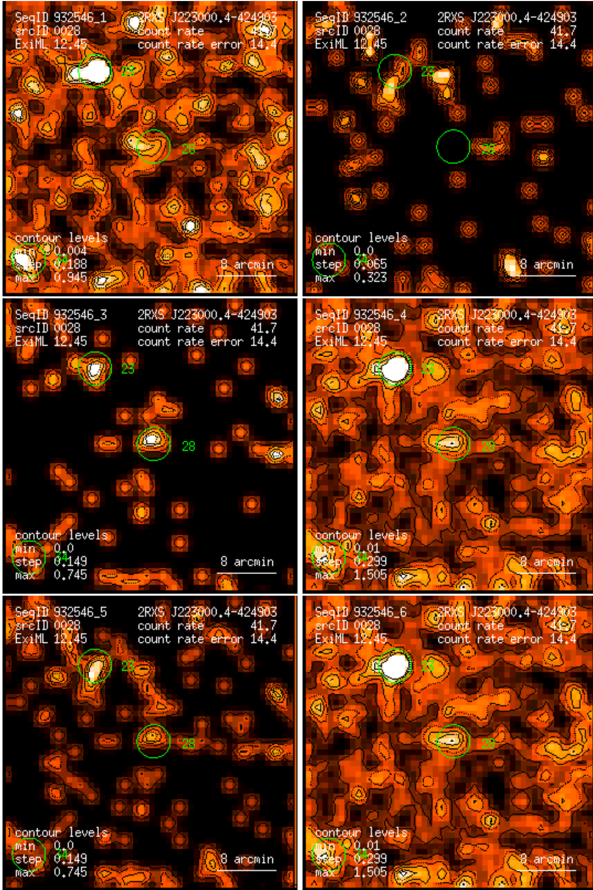
Figure 28: RASS 932546: detection 0028: band rate images, Gaussian filter: (1) PSPC channels 11 – 41, (2) 52 – 90, (3) 91 – 201, (4) 11 – 235, (5) 52 – 201, (6) 11 – 201. Broad band rates in counts/ks. Band rate contour levels in counts/ks/arcmin 2 .
