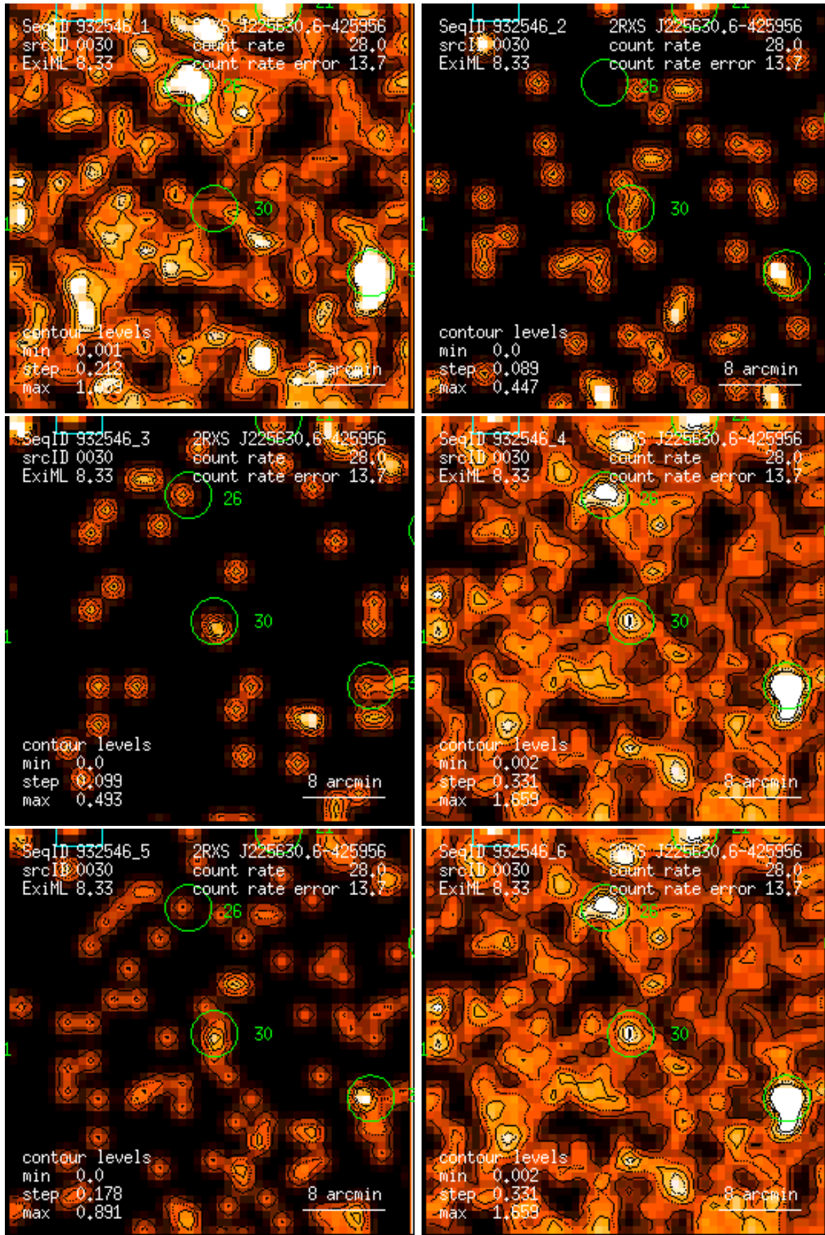
Figure 30: RASS 932546: detection 0030: band rate images, Gaussian filter: (1) PSPC channels 11 – 41, (2) 52 – 90, (3) 91 – 201, (4) 11 – 235, (5) 52 – 201, (6) 11 – 201. Broad band rates in counts/ks. Band rate contour levels in counts/ks/arcmin 2 .
