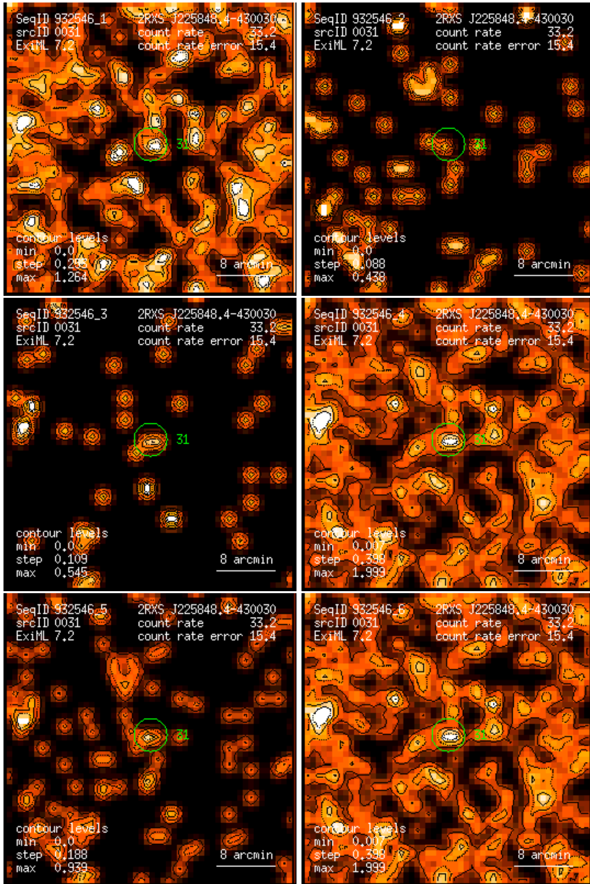
Figure 31: RASS 932546: detection 0031: band rate images, Gaussian filter: (1) PSPC channels 11 – 41, (2) 52 – 90, (3) 91 – 201, (4) 11 – 235, (5) 52 – 201, (6) 11 – 201. Broad band rates in counts/ks. Band rate contour levels in counts/ks/arcmin 2 .
