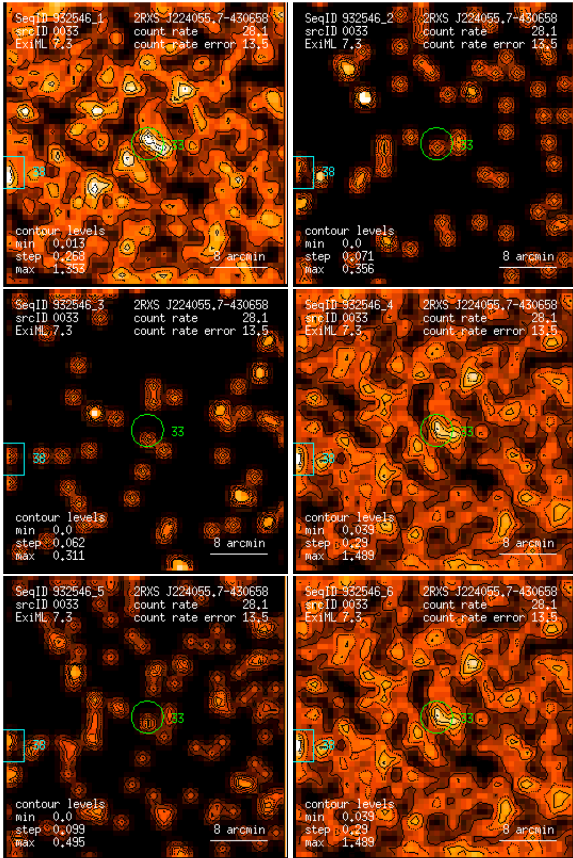
Figure 33: RASS 932546: detection 0033: band rate images, Gaussian filter: (1) PSPC channels 11 – 41, (2) 52 – 90, (3) 91 – 201, (4) 11 – 235, (5) 52 – 201, (6) 11 – 201. Broad band rates in counts/ks. Band rate contour levels in counts/ks/arcmin 2 .
