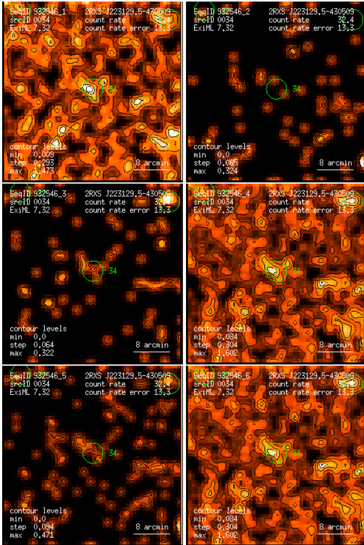
Figure 34: RASS 932546: detection 0034: band rate images, Gaussian filter: (1) PSPC channels 11 – 41, (2) 52 – 90, (3) 91 – 201, (4) 11 – 235, (5) 52 – 201, (6) 11 – 201. Broad band rates in counts/ks. Band rate contour levels in counts/ks/arcmin 2 .
