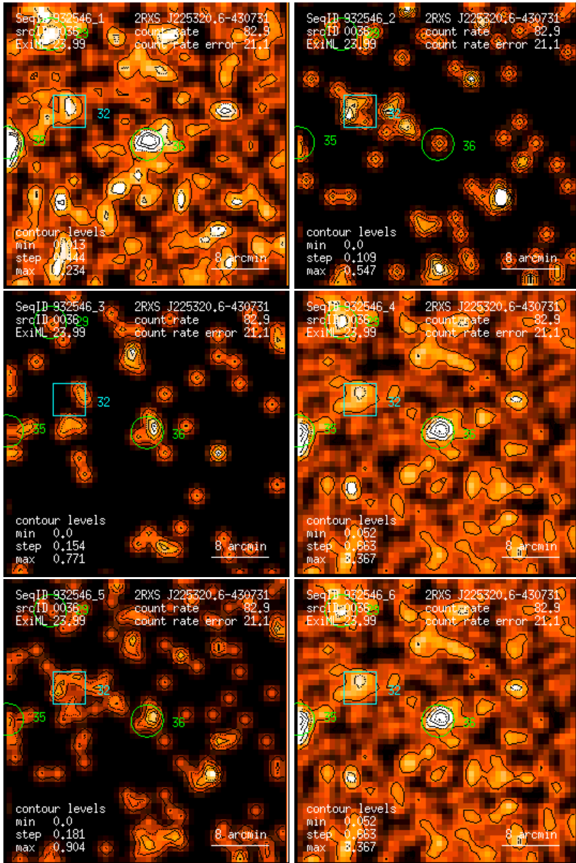
Figure 36: RASS 932546: detection 0036: band rate images, Gaussian filter: (1) PSPC channels 11 – 41, (2) 52 – 90, (3) 91 – 201, (4) 11 – 235, (5) 52 – 201, (6) 11 – 201. Broad band rates in counts/ks. Band rate contour levels in counts/ks/arcmin 2 .
