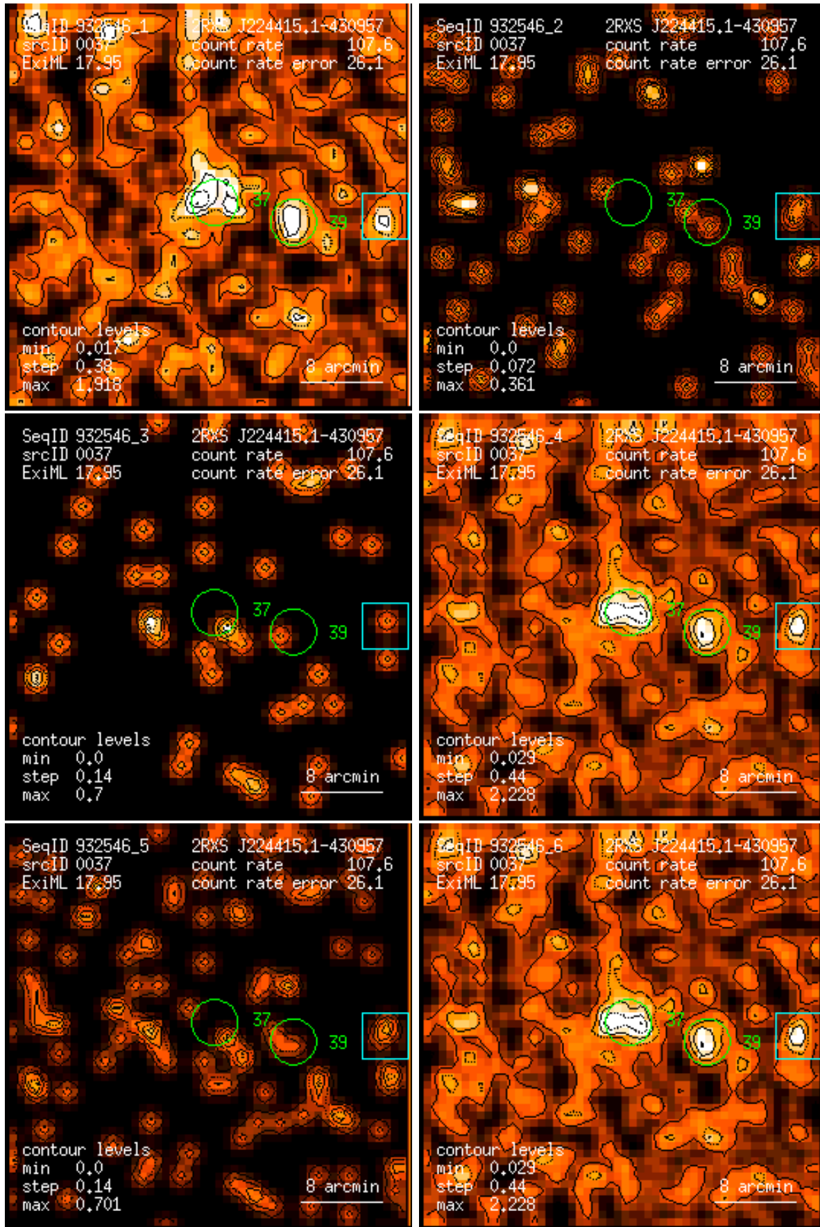
Figure 37: RASS 932546: detection 0037: band rate images, Gaussian filter: (1) PSPC channels 11 – 41, (2) 52 – 90, (3) 91 – 201, (4) 11 – 235, (5) 52 – 201, (6) 11 – 201. Broad band rates in counts/ks. Band rate contour levels in counts/ks/arcmin 2 .
