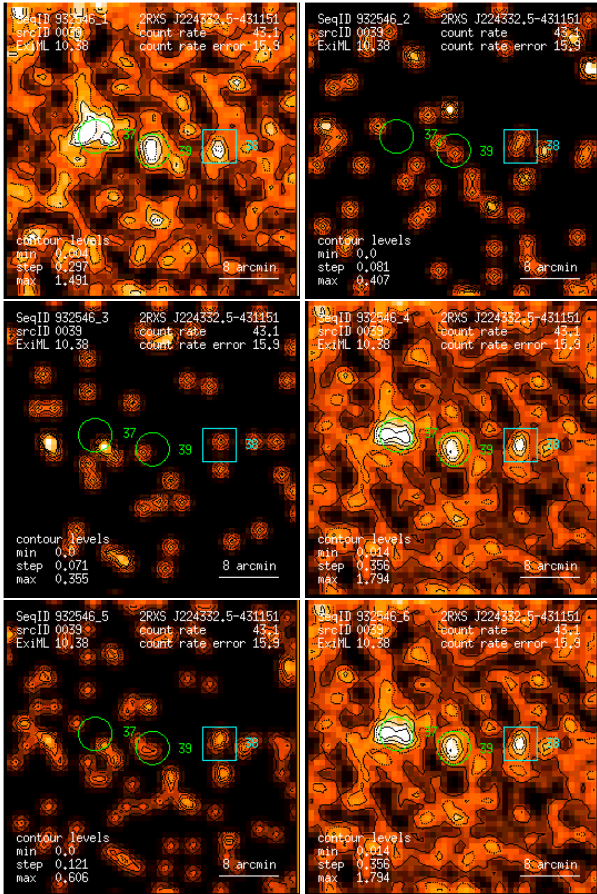
Figure 39: RASS 932546: detection 0039: band rate images, Gaussian filter: (1) PSPC channels 11 – 41, (2) 52 – 90, (3) 91 – 201, (4) 11 – 235, (5) 52 – 201, (6) 11 – 201. Broad band rates in counts/ks. Band rate contour levels in counts/ks/arcmin 2 .
