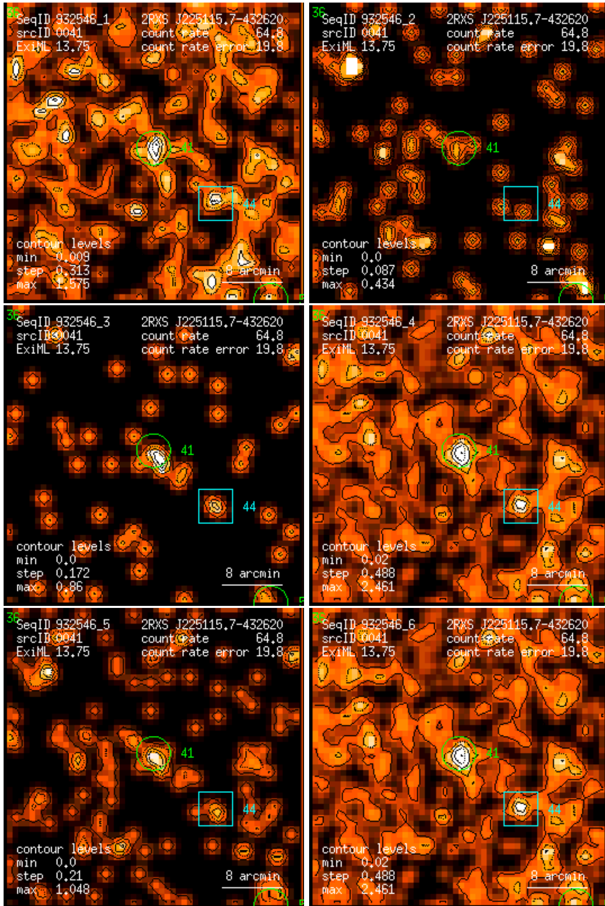
Figure 41: RASS 932546: detection 0041: band rate images, Gaussian filter: (1) PSPC channels 11 – 41, (2) 52 – 90, (3) 91 – 201, (4) 11 – 235, (5) 52 – 201, (6) 11 – 201. Broad band rates in counts/ks. Band rate contour levels in counts/ks/arcmin 2 .
