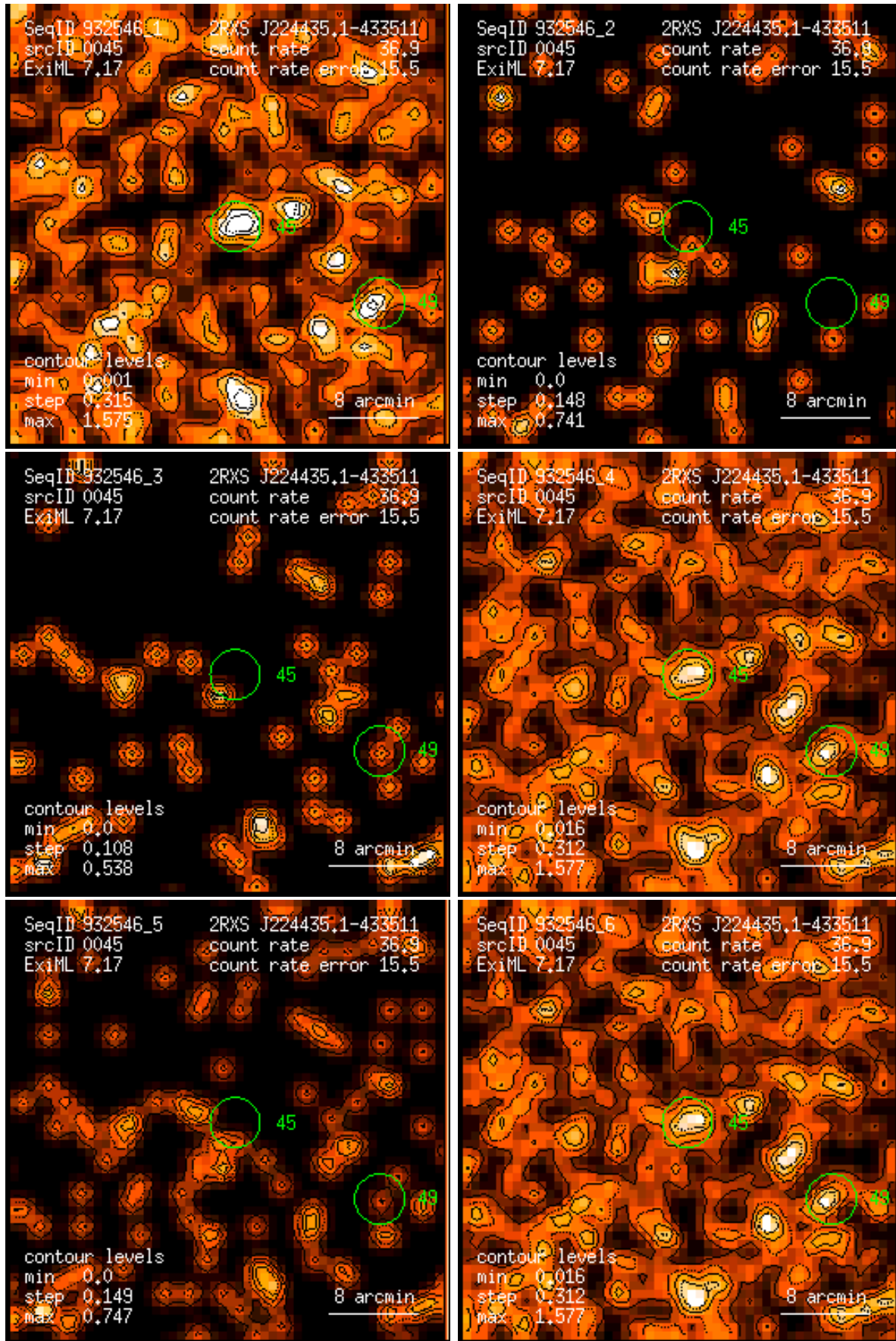
Figure 45: RASS 932546: detection 0045: band rate images, Gaussian filter: (1) PSPC channels 11 – 41, (2) 52 – 90, (3) 91 – 201, (4) 11 – 235, (5) 52 – 201, (6) 11 – 201. Broad band rates in counts/ks. Band rate contour levels in counts/ks/arcmin 2 .
