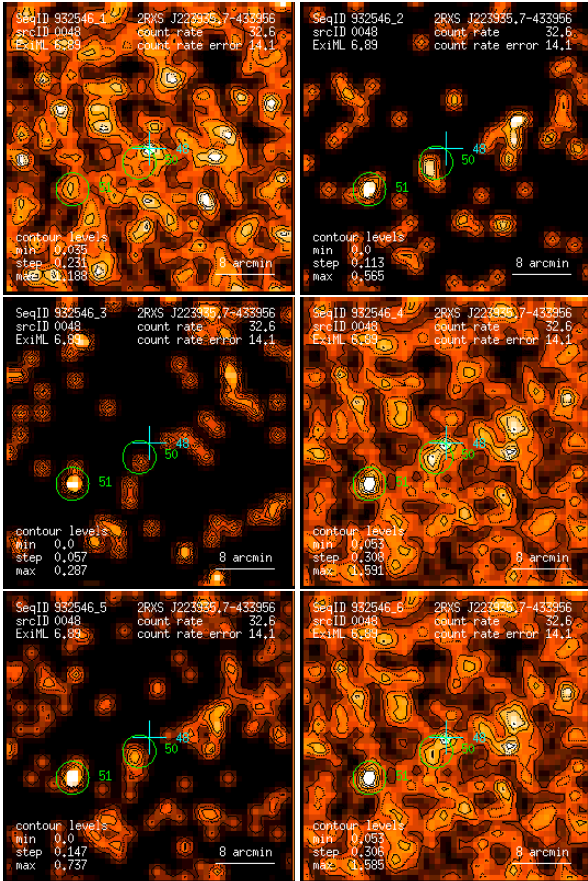
Figure 48: RASS 932546: detection 0048: band rate images, Gaussian filter: (1) PSPC channels 11 – 41, (2) 52 – 90, (3) 91 – 201, (4) 11 – 235, (5) 52 – 201, (6) 11 – 201. Broad band rates in counts/ks. Band rate contour levels in counts/ks/arcmin 2 .
