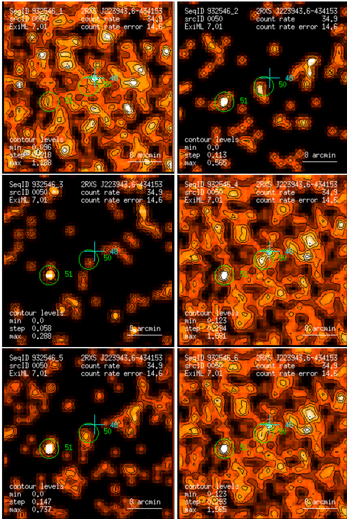
Figure 50: RASS 932546: detection 0050: band rate images, Gaussian filter: (1) PSPC channels 11 – 41, (2) 52 – 90, (3) 91 – 201, (4) 11 – 235, (5) 52 – 201, (6) 11 – 201. Broad band rates in counts/ks. Band rate contour levels in counts/ks/arcmin 2 .
