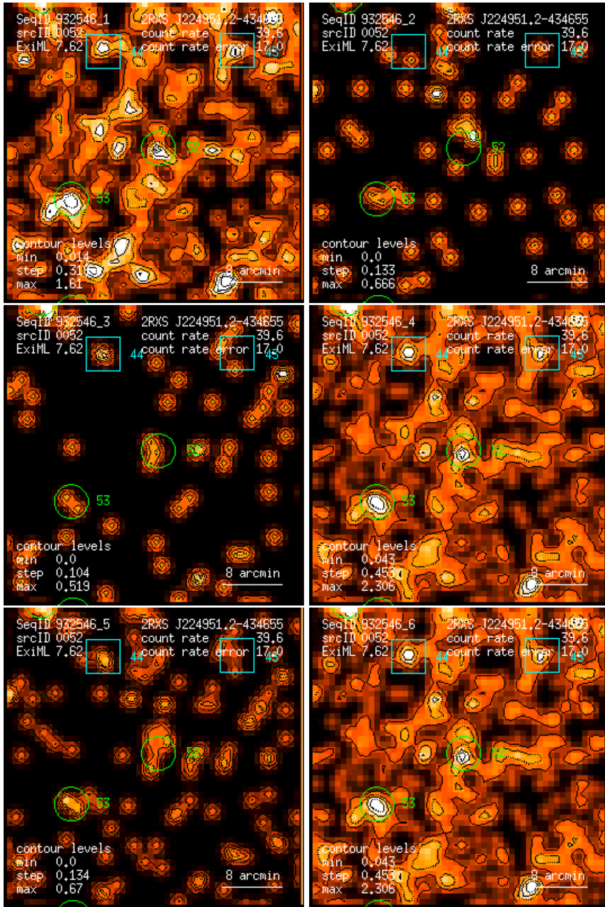
Figure 52: RASS 932546: detection 0052: band rate images, Gaussian filter: (1) PSPC channels 11 – 41, (2) 52 – 90, (3) 91 – 201, (4) 11 – 235, (5) 52 – 201, (6) 11 – 201. Broad band rates in counts/ks. Band rate contour levels in counts/ks/arcmin 2 .
