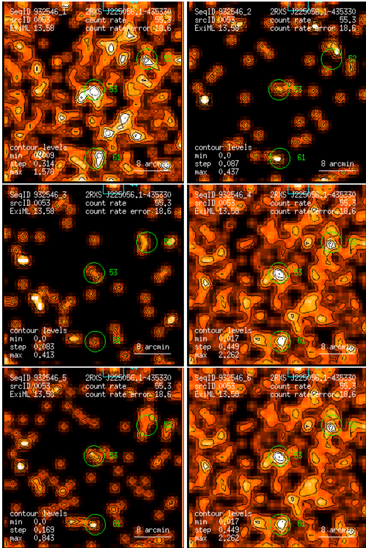
Figure 53: RASS 932546: detection 0053: band rate images, Gaussian filter: (1) PSPC channels 11 – 41, (2) 52 – 90, (3) 91 – 201, (4) 11 – 235, (5) 52 – 201, (6) 11 – 201. Broad band rates in counts/ks. Band rate contour levels in counts/ks/arcmin 2 .
