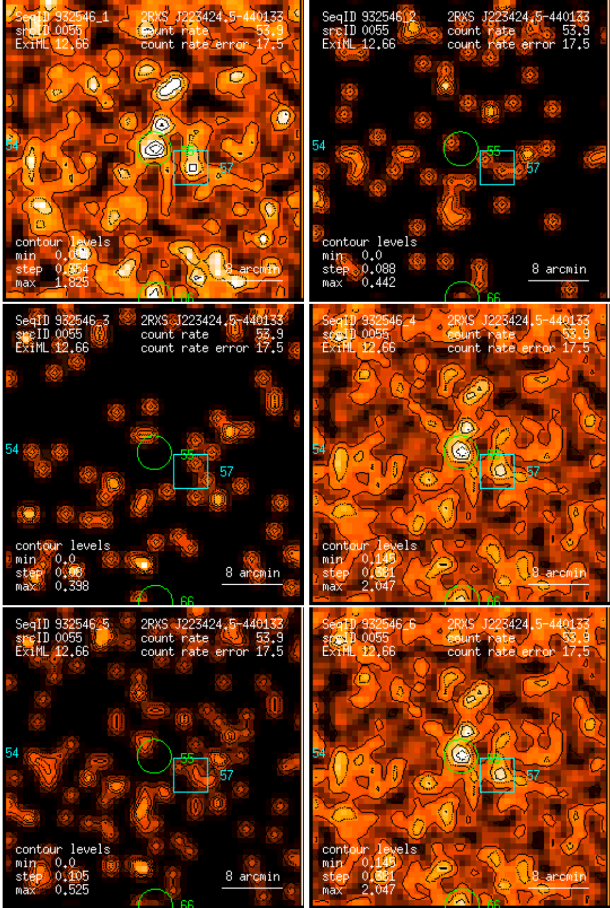
Figure 55: RASS 932546: detection 0055: band rate images, Gaussian filter: (1) PSPC channels 11 – 41, (2) 52 – 90, (3) 91 – 201, (4) 11 – 235, (5) 52 – 201, (6) 11 – 201. Broad band rates in counts/ks. Band rate contour levels in counts/ks/arcmin 2 .
