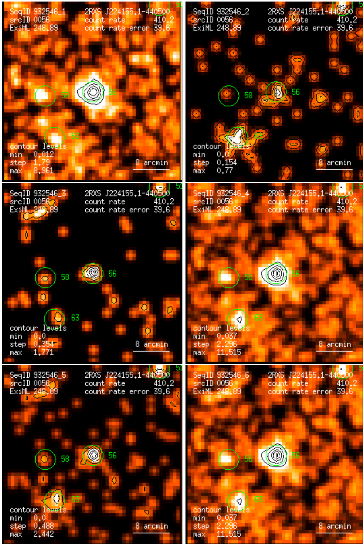
Figure 56: RASS 932546: detection 0056: band rate images, Gaussian filter: (1) PSPC channels 11 – 41, (2) 52 – 90, (3) 91 – 201, (4) 11 – 235, (5) 52 – 201, (6) 11 – 201. Broad band rates in counts/ks. Band rate contour levels in counts/ks/arcmin 2 .
