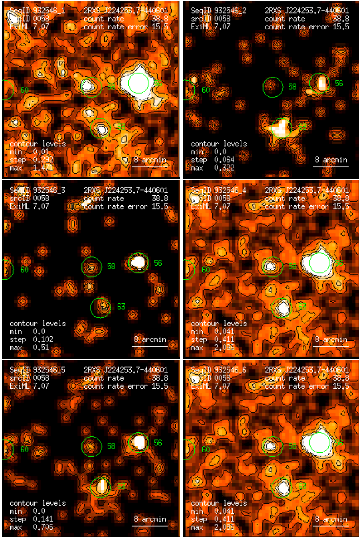
Figure 58: RASS 932546: detection 0058: band rate images, Gaussian filter: (1) PSPC channels 11 – 41, (2) 52 – 90, (3) 91 – 201, (4) 11 – 235, (5) 52 – 201, (6) 11 – 201. Broad band rates in counts/ks. Band rate contour levels in counts/ks/arcmin 2 .
