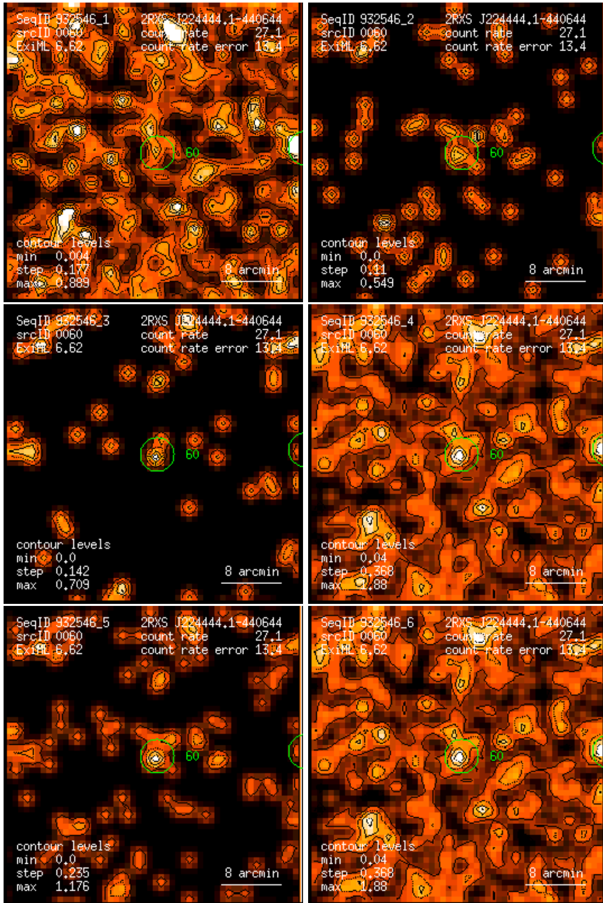
Figure 60: RASS 932546: detection 0060: band rate images, Gaussian filter: (1) PSPC channels 11 – 41, (2) 52 – 90, (3) 91 – 201, (4) 11 – 235, (5) 52 – 201, (6) 11 – 201. Broad band rates in counts/ks. Band rate contour levels in counts/ks/arcmin 2 .
