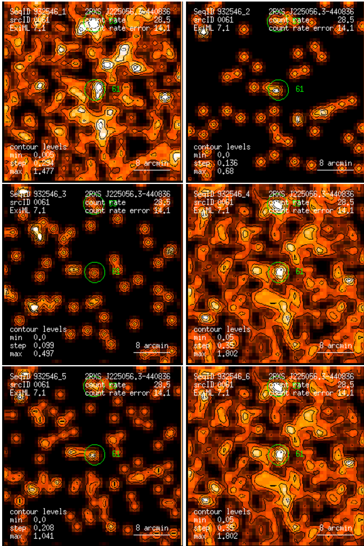
Figure 61: RASS 932546: detection 0061: band rate images, Gaussian filter: (1) PSPC channels 11 – 41, (2) 52 – 90, (3) 91 – 201, (4) 11 – 235, (5) 52 – 201, (6) 11 – 201. Broad band rates in counts/ks. Band rate contour levels in counts/ks/arcmin 2 .
