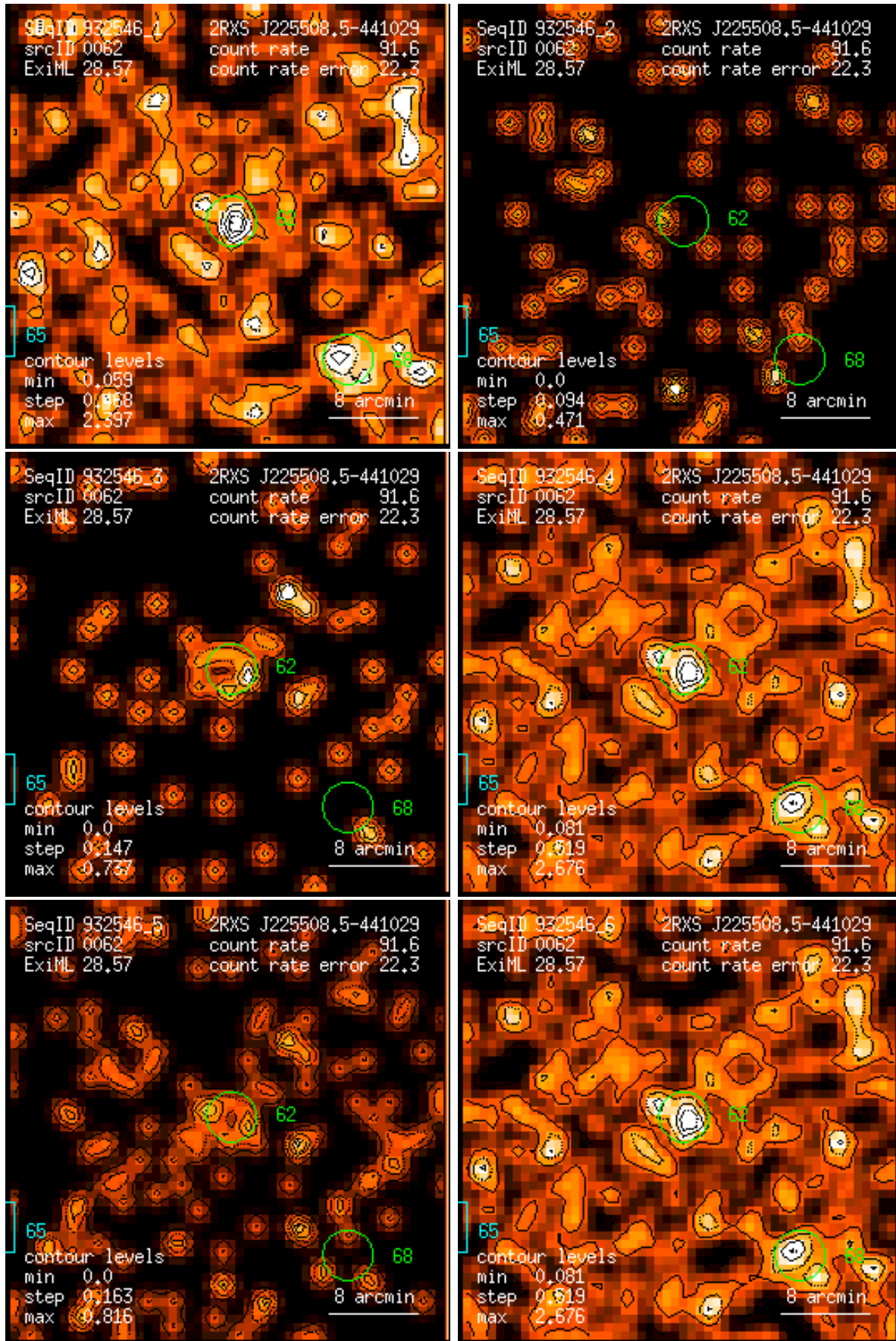
Figure 62: RASS 932546: detection 0062: band rate images, Gaussian filter: (1) PSPC channels 11 – 41, (2) 52 – 90, (3) 91 – 201, (4) 11 – 235, (5) 52 – 201, (6) 11 – 201. Broad band rates in counts/ks. Band rate contour levels in counts/ks/arcmin 2 .
