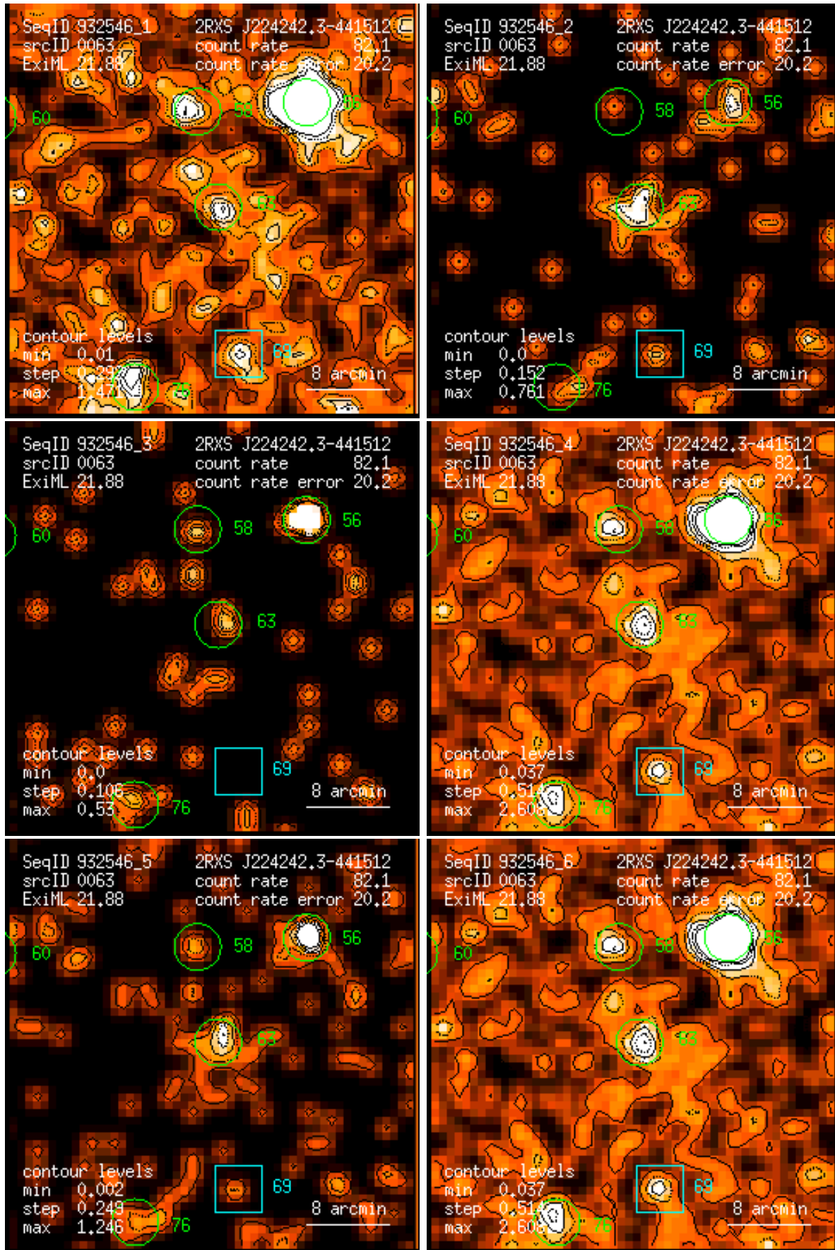
Figure 63: RASS 932546: detection 0063: band rate images, Gaussian filter: (1) PSPC channels 11 – 41, (2) 52 – 90, (3) 91 – 201, (4) 11 – 235, (5) 52 – 201, (6) 11 – 201. Broad band rates in counts/ks. Band rate contour levels in counts/ks/arcmin 2 .
