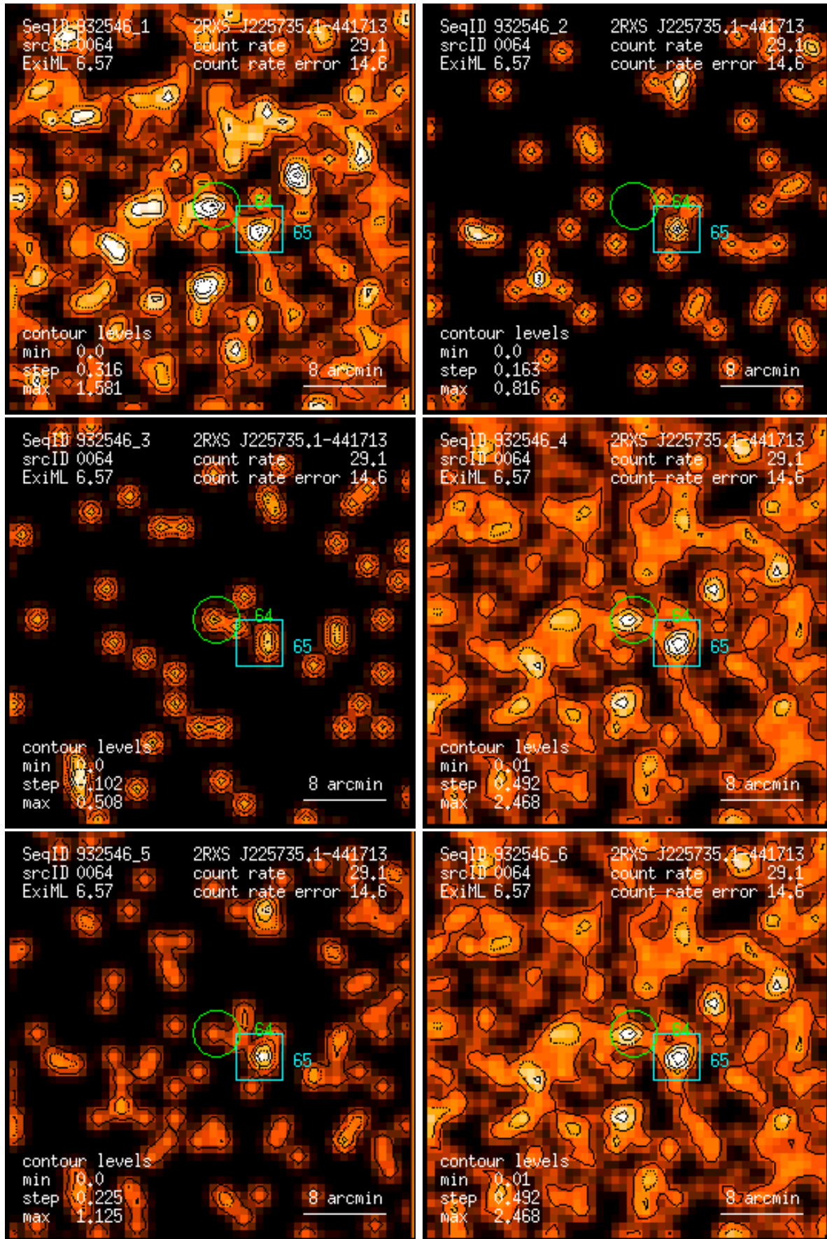
Figure 64: RASS 932546: detection 0064: band rate images, Gaussian filter: (1) PSPC channels 11 – 41, (2) 52 – 90, (3) 91 – 201, (4) 11 – 235, (5) 52 – 201, (6) 11 – 201. Broad band rates in counts/ks. Band rate contour levels in counts/ks/arcmin 2 .
