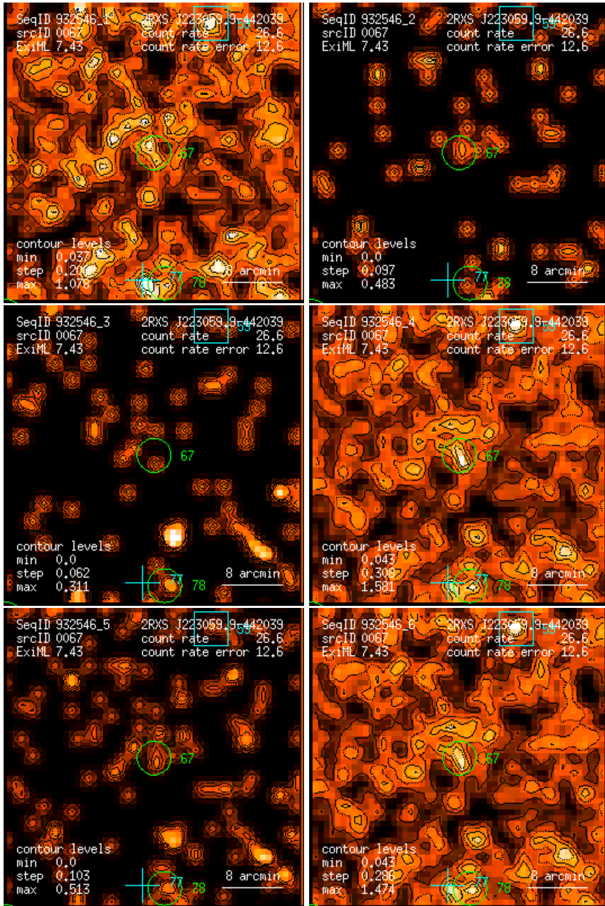
Figure 67: RASS 932546: detection 0067: band rate images, Gaussian filter: (1) PSPC channels 11 – 41, (2) 52 – 90, (3) 91 – 201, (4) 11 – 235, (5) 52 – 201, (6) 11 – 201. Broad band rates in counts/ks. Band rate contour levels in counts/ks/arcmin 2 .
