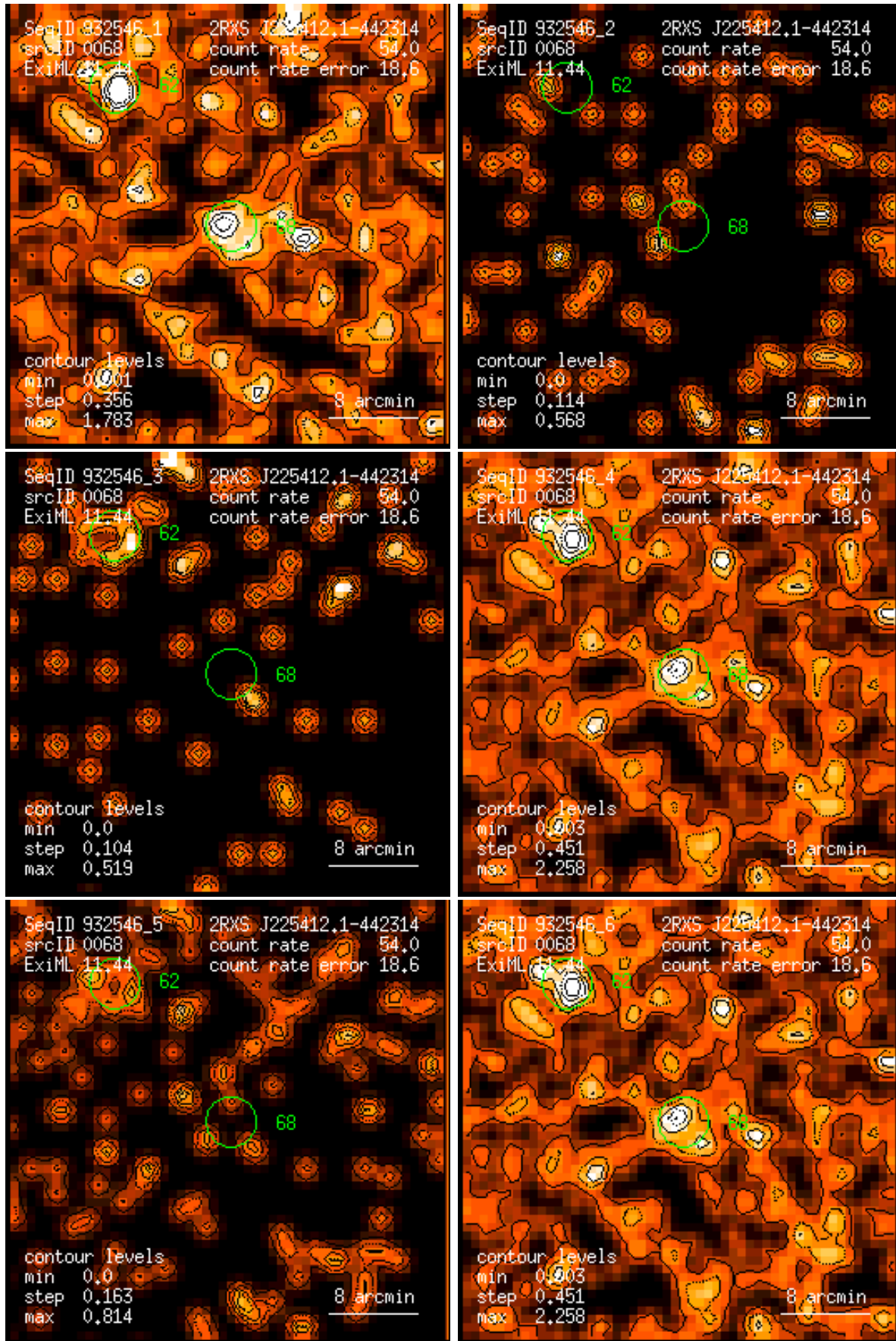
Figure 68: RASS 932546: detection 0068: band rate images, Gaussian filter: (1) PSPC channels 11 – 41, (2) 52 – 90, (3) 91 – 201, (4) 11 – 235, (5) 52 – 201, (6) 11 – 201. Broad band rates in counts/ks. Band rate contour levels in counts/ks/arcmin 2 .
