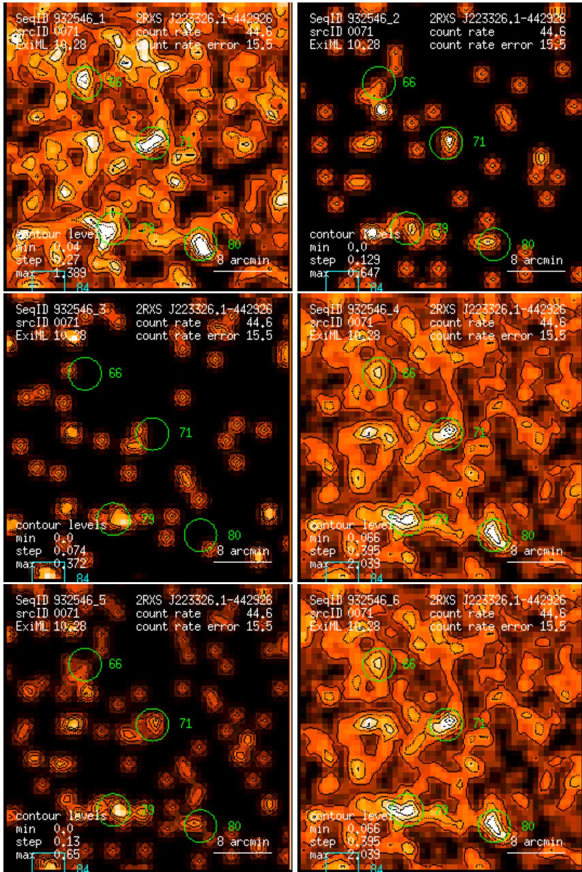
Figure 71: RASS 932546: detection 0071: band rate images, Gaussian filter: (1) PSPC channels 11 – 41, (2) 52 – 90, (3) 91 – 201, (4) 11 – 235, (5) 52 – 201, (6) 11 – 201. Broad band rates in counts/ks. Band rate contour levels in counts/ks/arcmin 2 .
