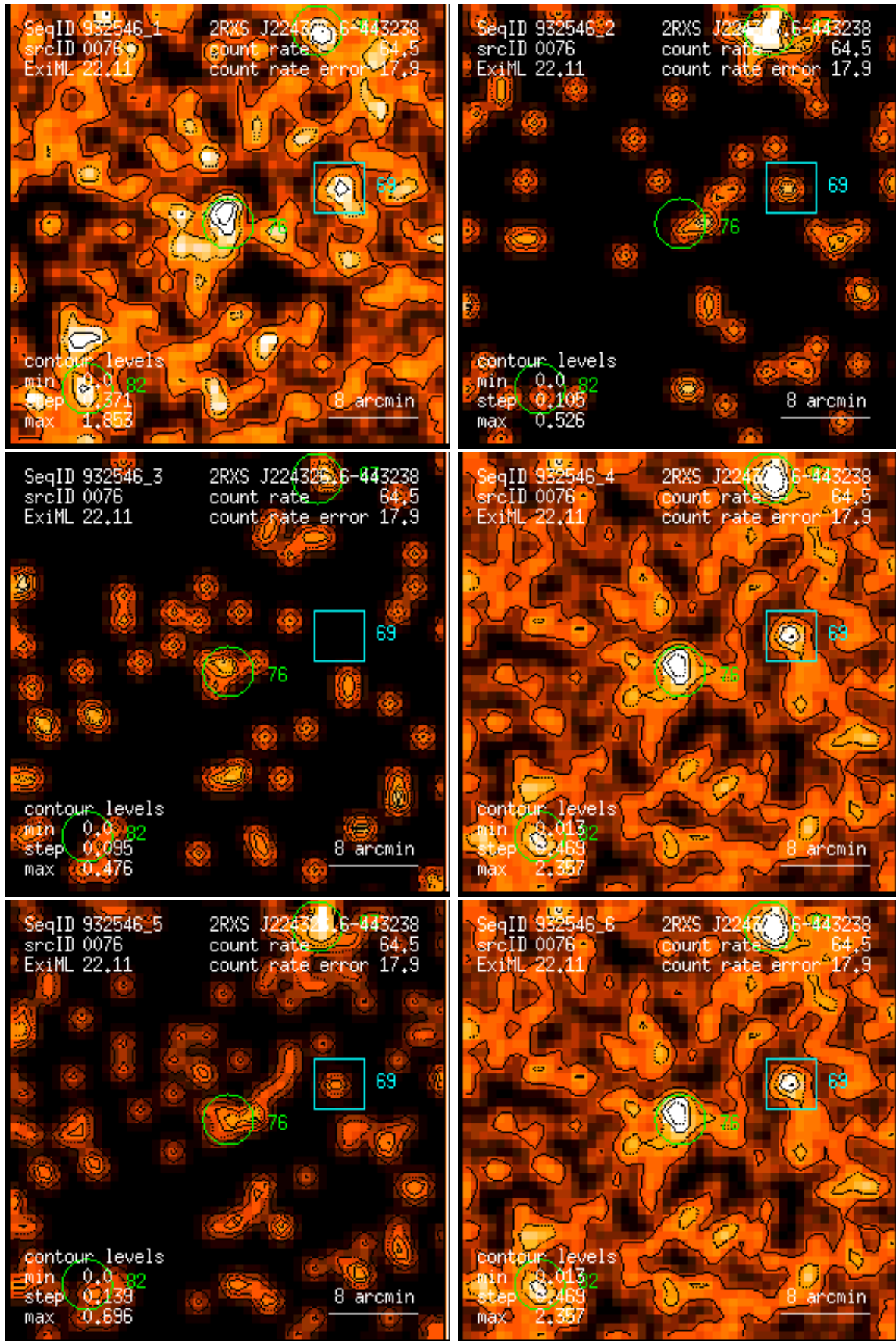
Figure 76: RASS 932546: detection 0076: band rate images, Gaussian filter: (1) PSPC channels 11 – 41, (2) 52 – 90, (3) 91 – 201, (4) 11 – 235, (5) 52 – 201, (6) 11 – 201. Broad band rates in counts/ks. Band rate contour levels in counts/ks/arcmin 2 .
