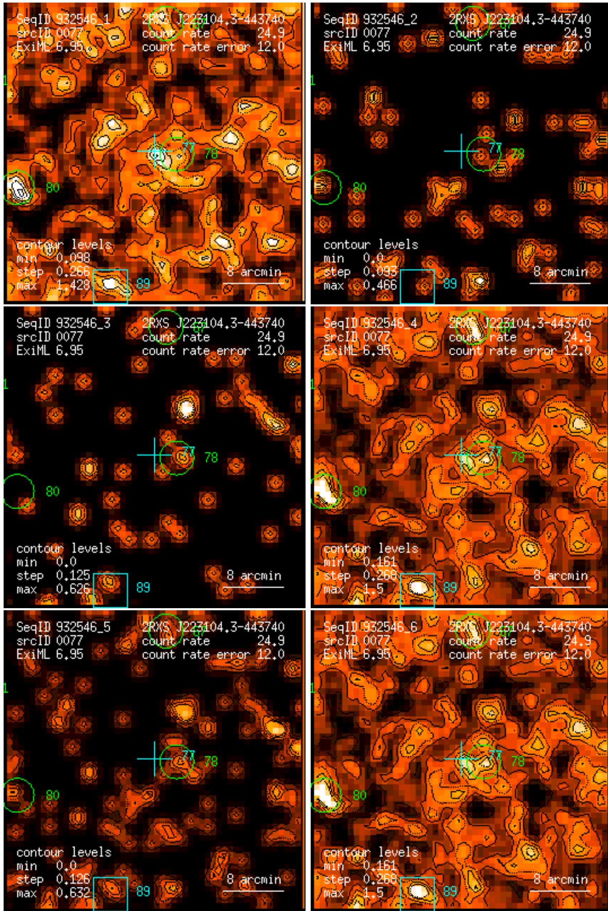
Figure 77: RASS 932546: detection 0077: band rate images, Gaussian filter: (1) PSPC channels 11 – 41, (2) 52 – 90, (3) 91 – 201, (4) 11 – 235, (5) 52 – 201, (6) 11 – 201. Broad band rates in counts/ks. Band rate contour levels in counts/ks/arcmin 2 .
