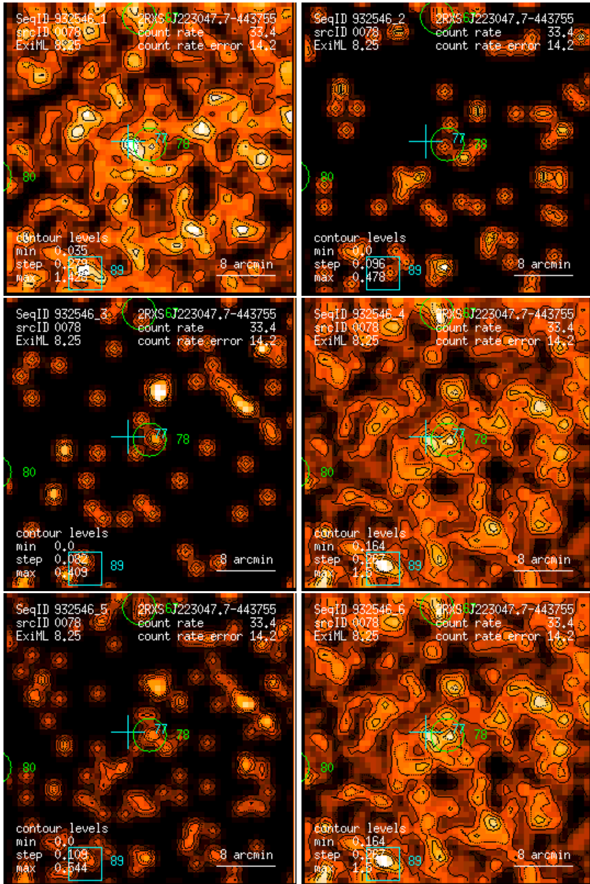
Figure 78: RASS 932546: detection 0078: band rate images, Gaussian filter: (1) PSPC channels 11 – 41, (2) 52 – 90, (3) 91 – 201, (4) 11 – 235, (5) 52 – 201, (6) 11 – 201. Broad band rates in counts/ks. Band rate contour levels in counts/ks/arcmin 2 .
